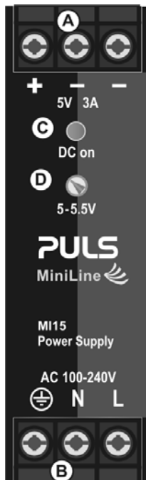
Fig. 10-1 Front side
