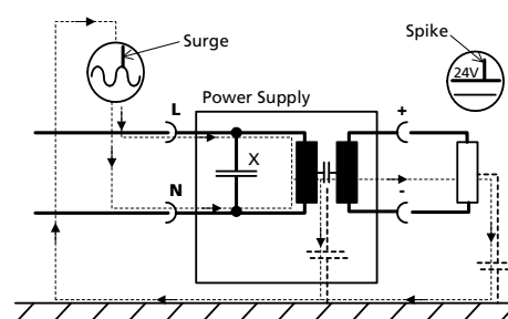
Fig. 21-4 Not earthed input
