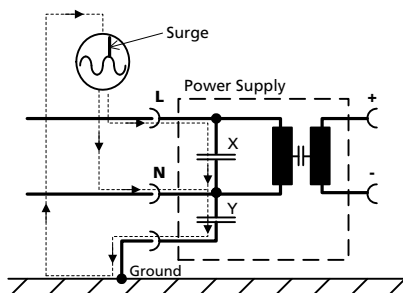
Fig. 21-3 Earthed input
