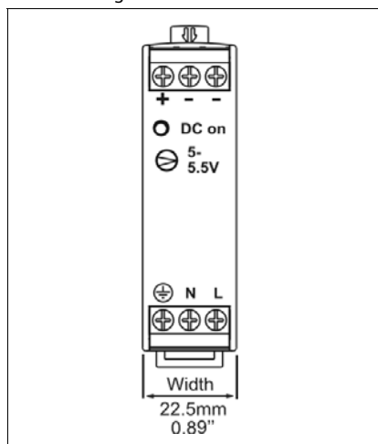
Fig. 20-1 Front view
