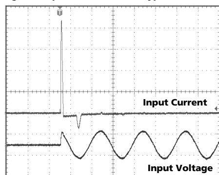
Fig. 5-1 Input inrush current, typical behavior
