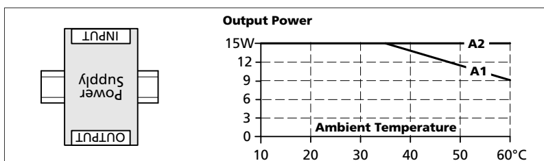
Fig. 21-6 Mounting Orientation B (Upside down)
