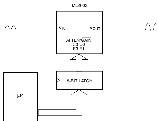
Figure 13. Typical \mu P Parallel Interface
