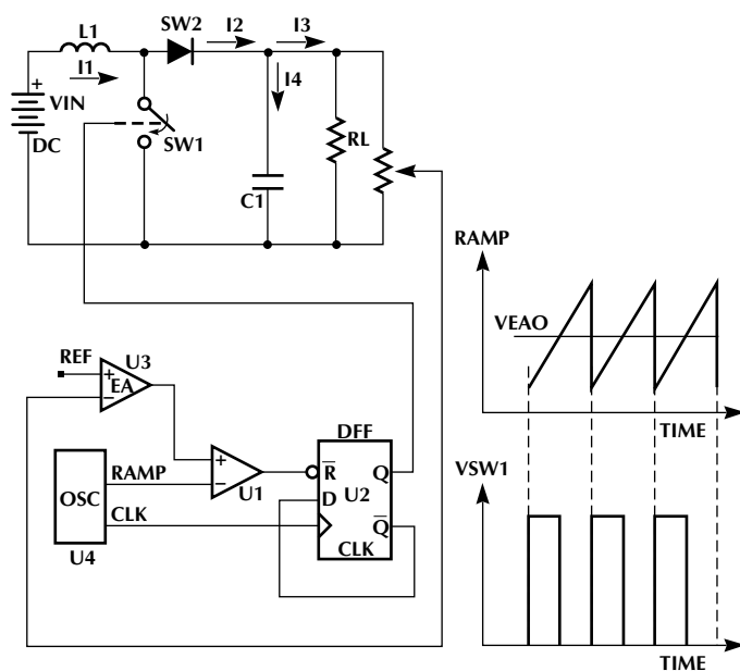
Figure 8. Typical Trailing Edge Control Scheme.
