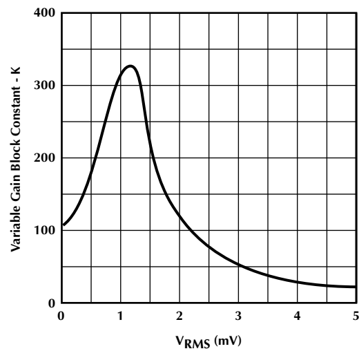
Variable Gain Control Transfer Characteristic
