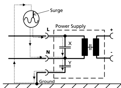
Fig. 22-5 Earthed input
