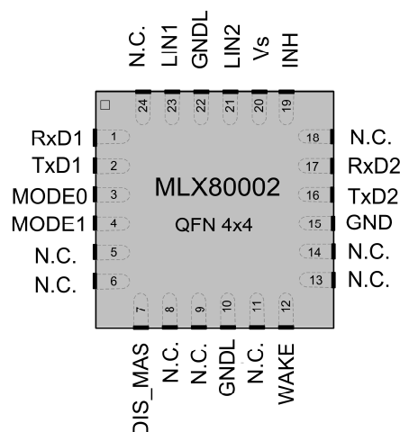
Figure 3: Pinout MLX80002 QFN24 package
