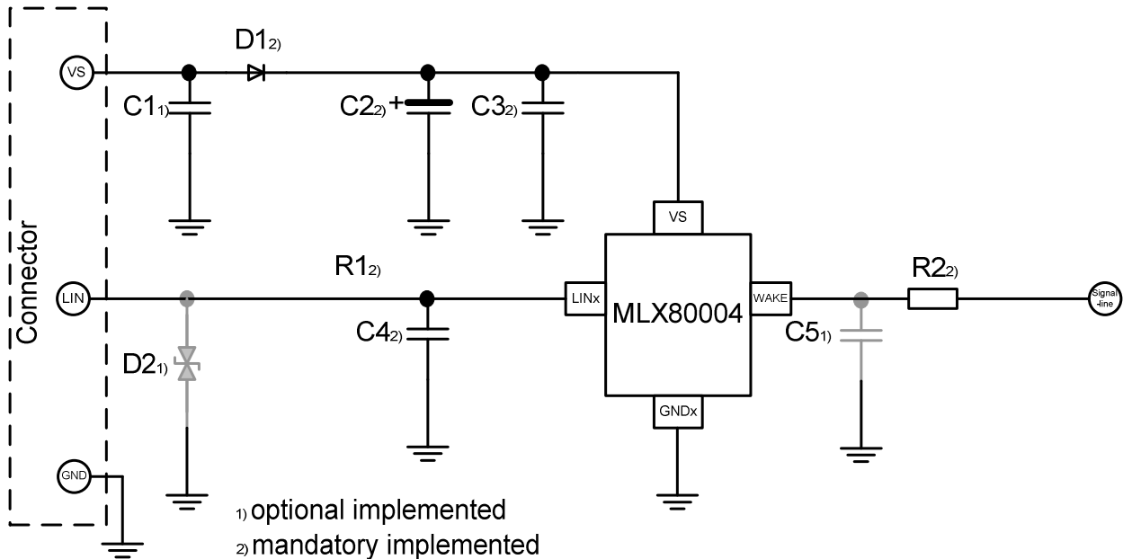
Figure 11: Typical Application Circuitry for EMC
