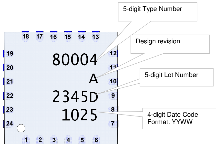
Figure 13: Package marking of the MLX80004 device in QFN24 4x4 SMD package
