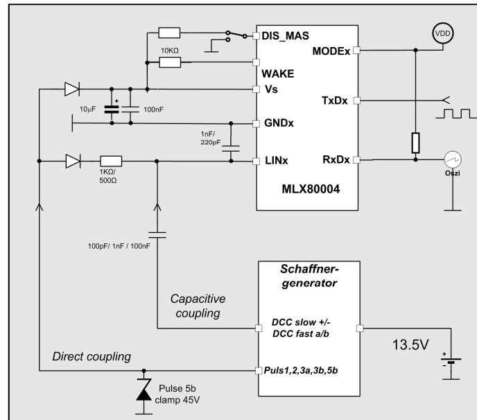
Figure 14: Test circuit for automotive transients
