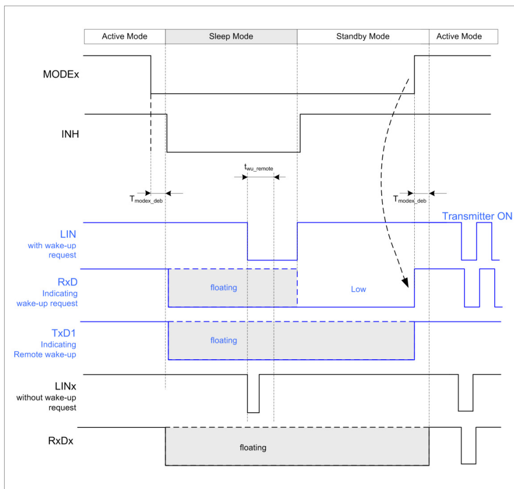
Figure 7: remote wake up and wake-up source recognition
