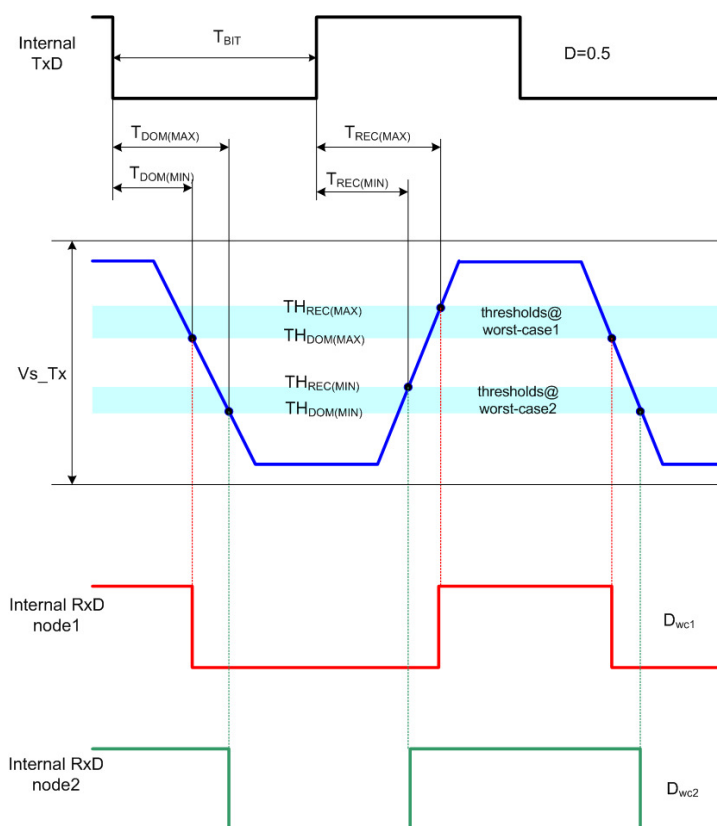
Figure 5: LIN timing diagram, relation between propagation delay and duty cycle (reference SAE J2602 specification)
