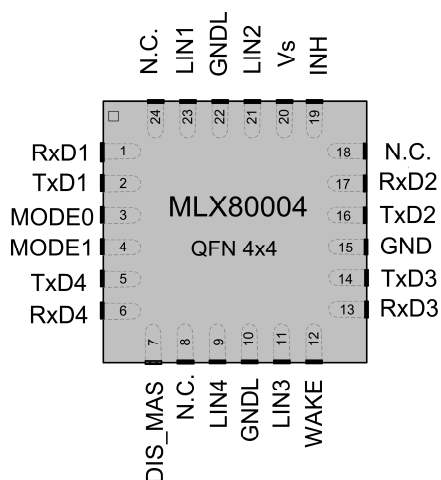
Figure 2: Pinout MLX80004 QFN24 package
