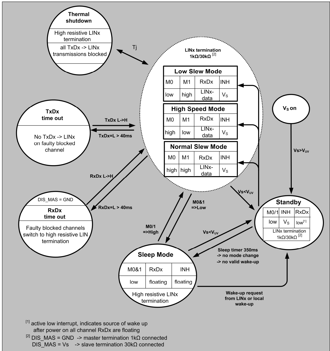
Figure 6: State Diagram of the MLX80004/2
