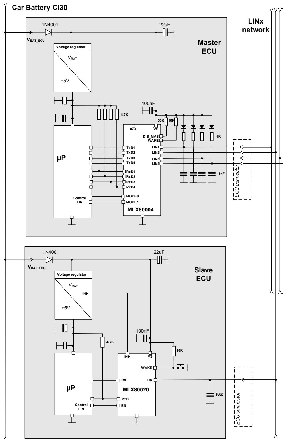
Figure 10: Application example using standard transceiver mode without LIN short to GND feature. Note: All pins of MLX80004/MLX80002 with „N.C.” must not be connected to a fixed potential on the PCB. Please keep them not connected.
