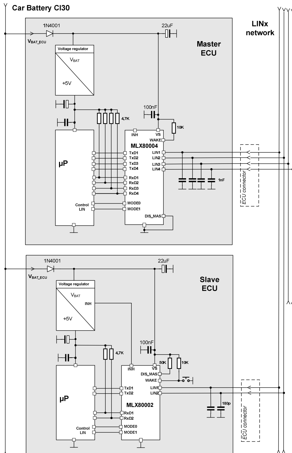
Figure 9: Application example using enhanced master mode with minimized external components and LIN short to GND feature. Note: All pins of MLX80004/MLX80002 with „N.C.“ must not be connected to a fixed potential on the PCB. Please keep them not connected.
