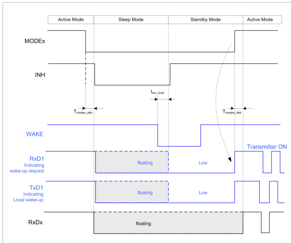
Figure 8: local wake up and wake-up source recognition
