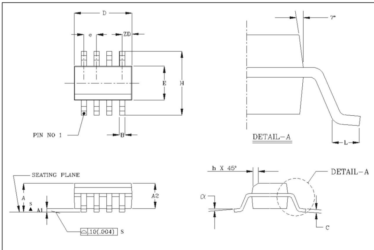
Figure 18: SOIC8 Drawing
