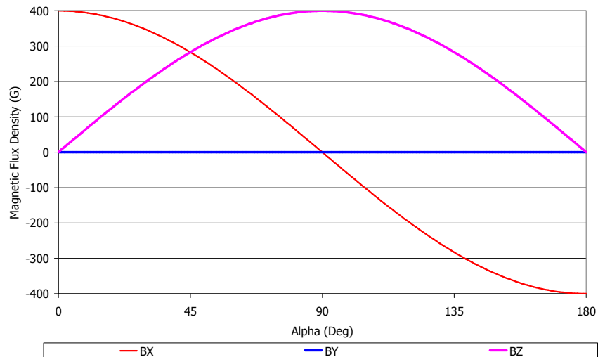
Figure 6 – Magnetic Flux Density – \beta = 90^\circ Deg – B_X \propto \cos(\alpha) , B_Y = 0 & B_Z \propto \sin(\alpha)
