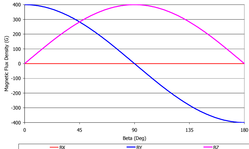
Figure 7 – Magnetic Flux Density – \alpha = 0^\circ Deg – B_X = 0 , B_Y \propto \cos(\beta) & B_Z \propto \sin(\beta)
