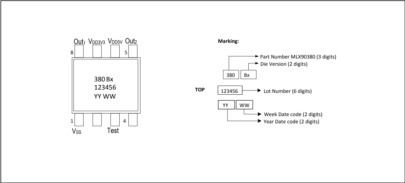
Figure 17: SOIC-8 Pin out and Marking
