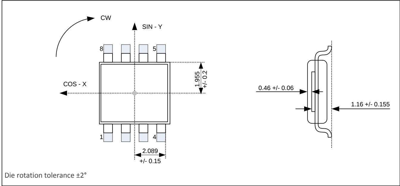
Figure 18: SOIC-8 IMC positioning
