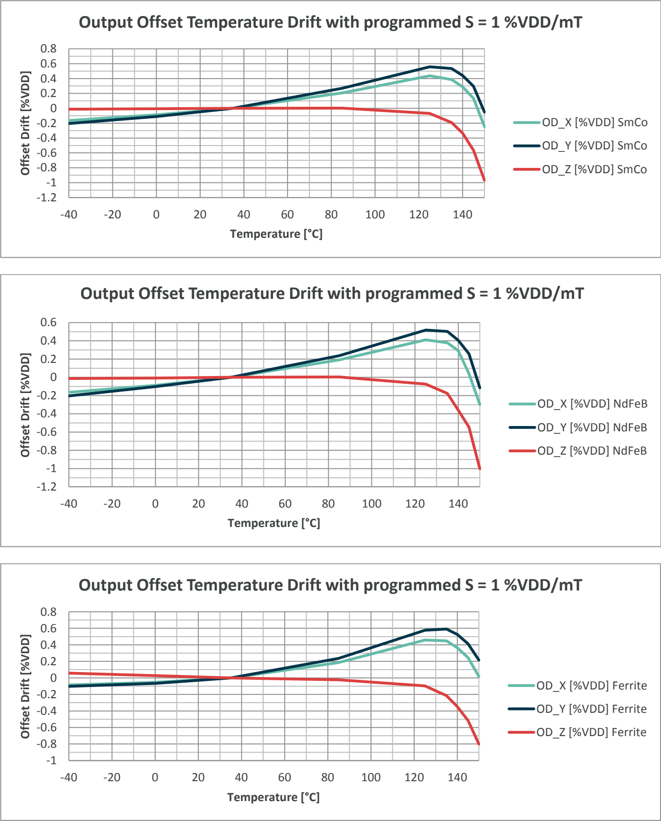
Figure 10: Output Offset Temperature Drift
