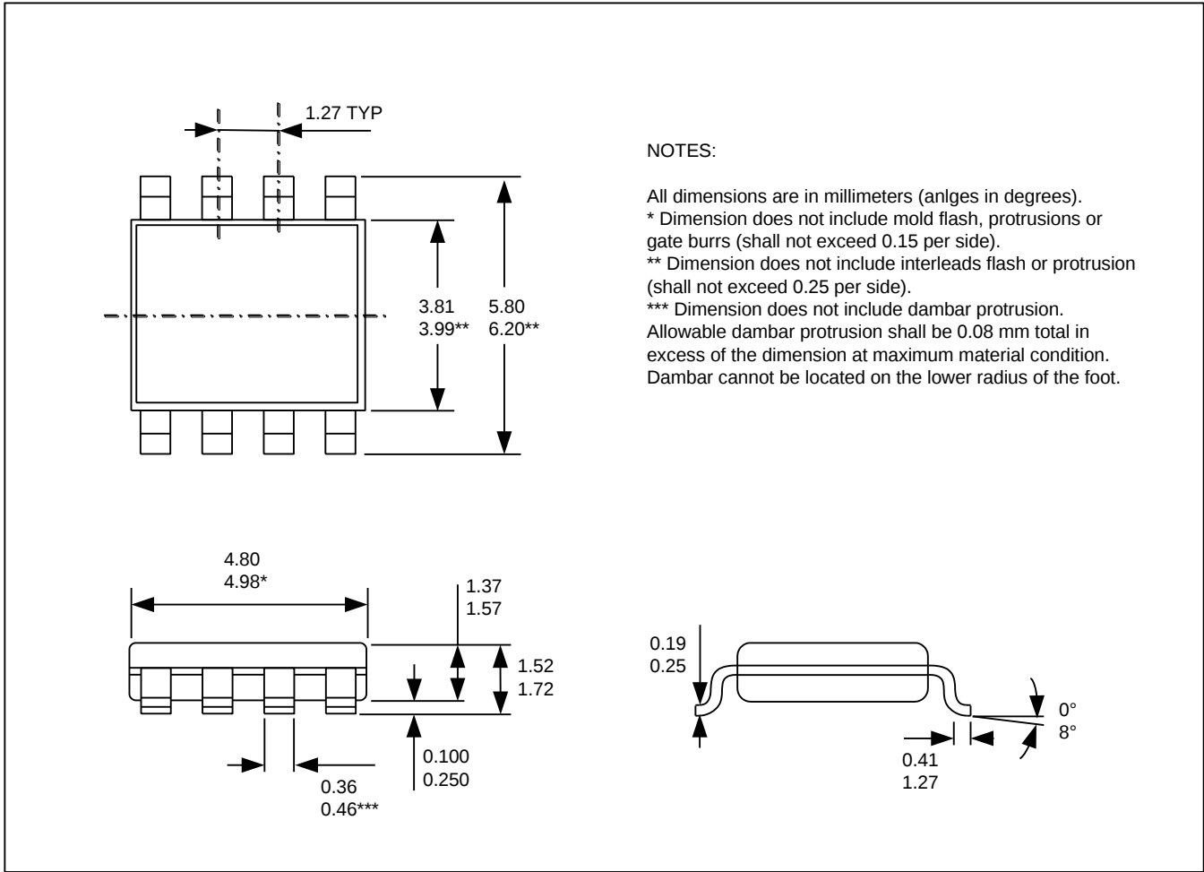
Figure 16: SOIC-8 Package Dimensions
