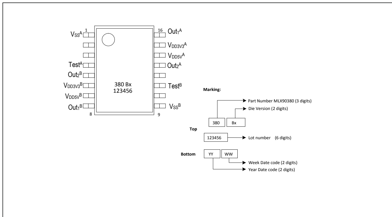
Figure 21: TSSOP-16 Pin out and Marking
