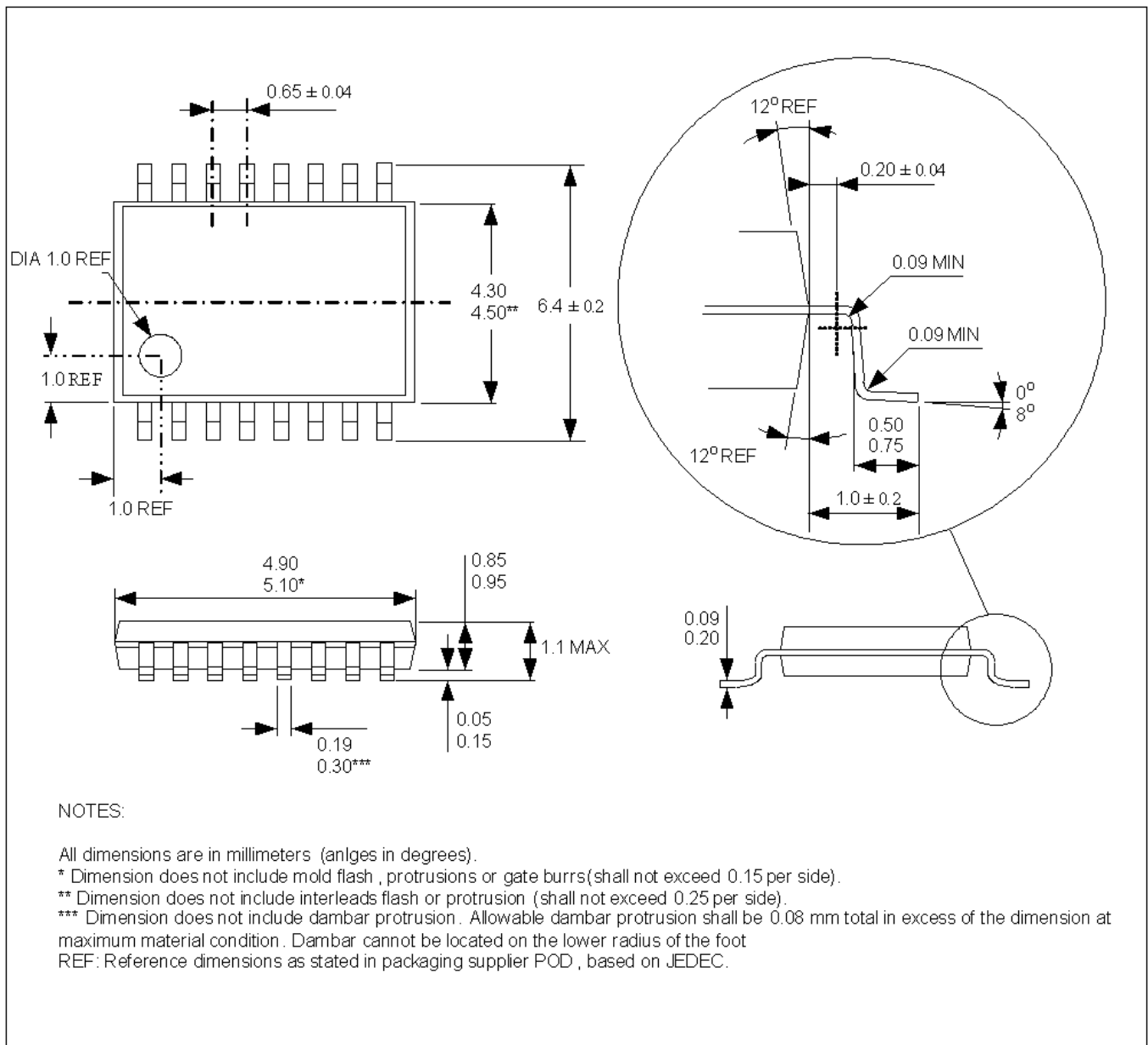
Figure 20: TSSOP-16 Package Dimensions
