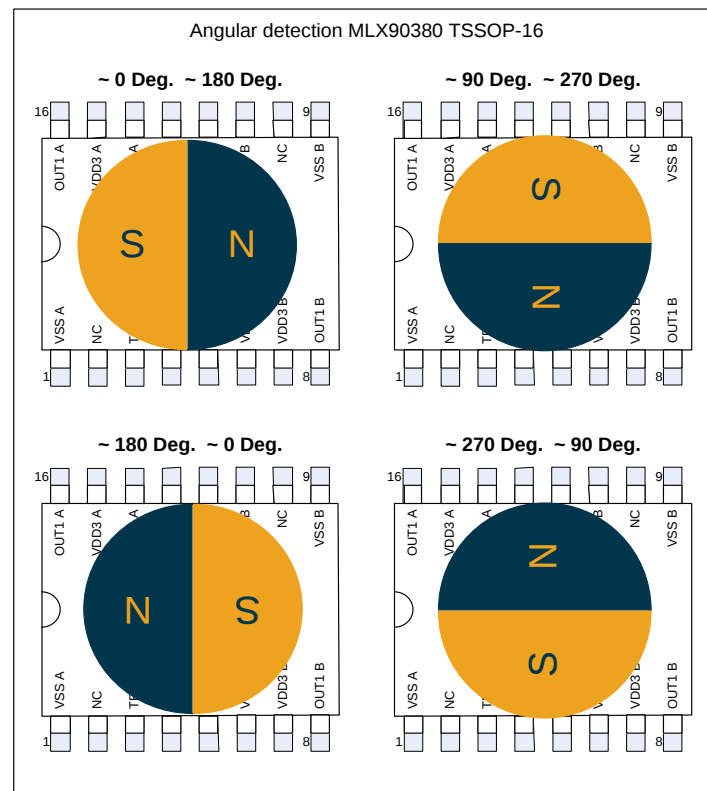
Figure 23: Angular detection MLX90380 TSSOP-16
