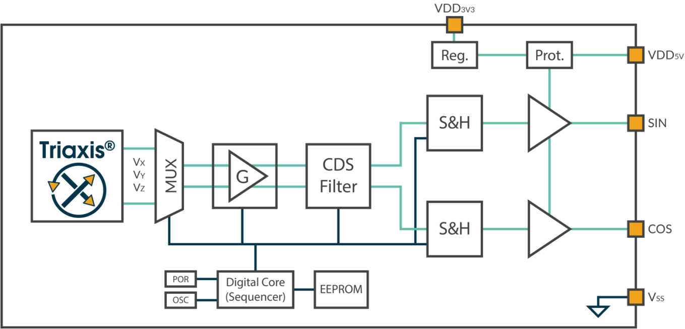
Figure 3: Functional Diagram
