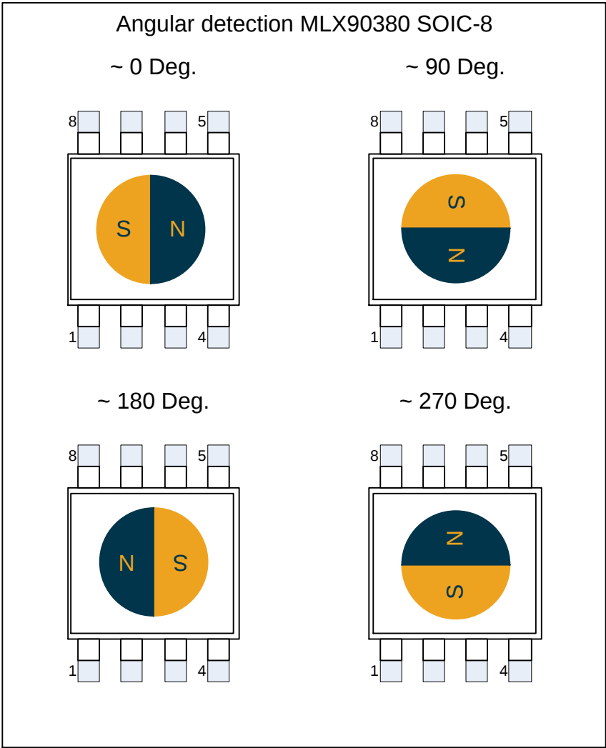
Figure 19: Angular detection MLX90380 SOIC-8
