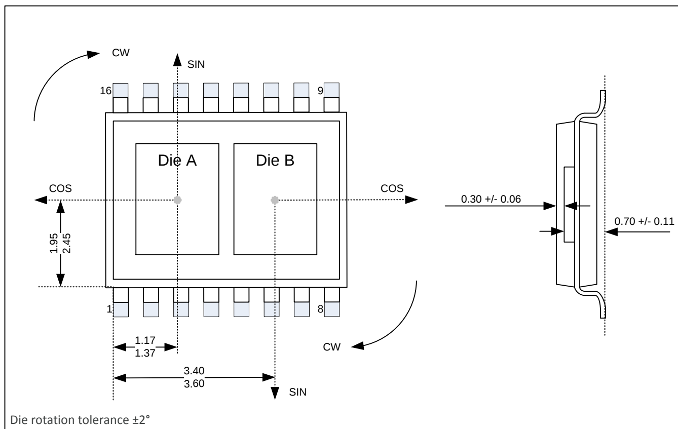
Figure 22: TSSOP-16 IMC positioning
