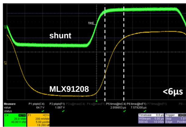
Figure 13: Response time with noise filter ON.
