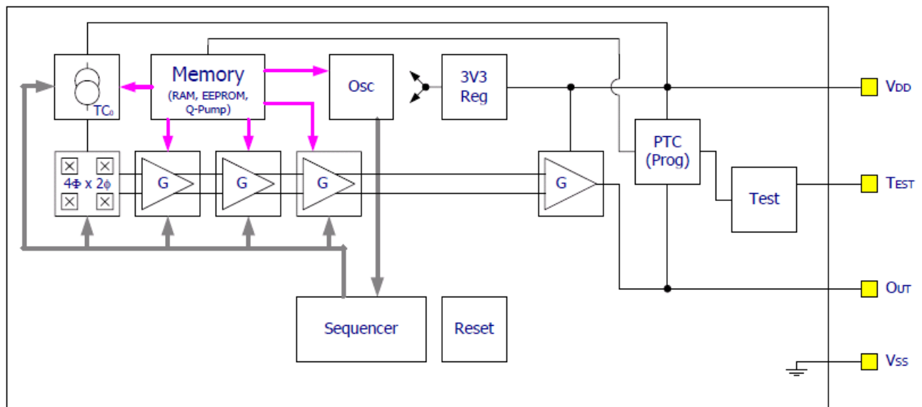
Figure 1: Block diagram
