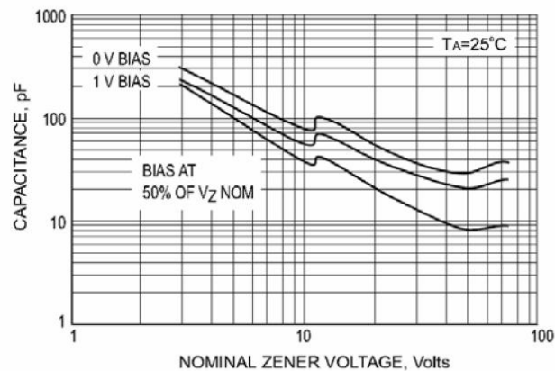
Fig.4 TYPICAL CAPACITANCE
