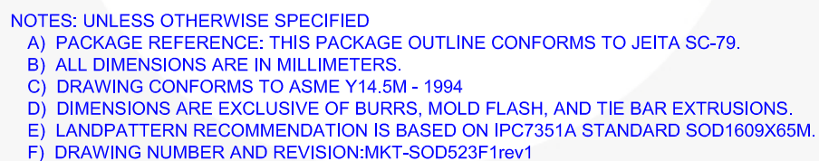
Figure 1. 2-LEAD, SOD523F, JEITA SC79, 0.7 MM TALL
