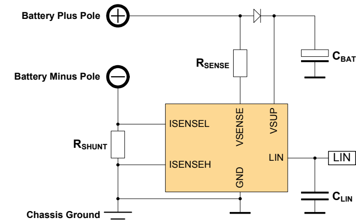
Figure 12. Typical IBS Application (Device GND = Chassis GND)
