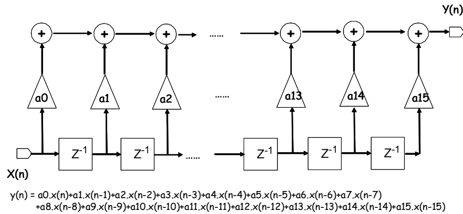
Figure 34. FIR Structure
