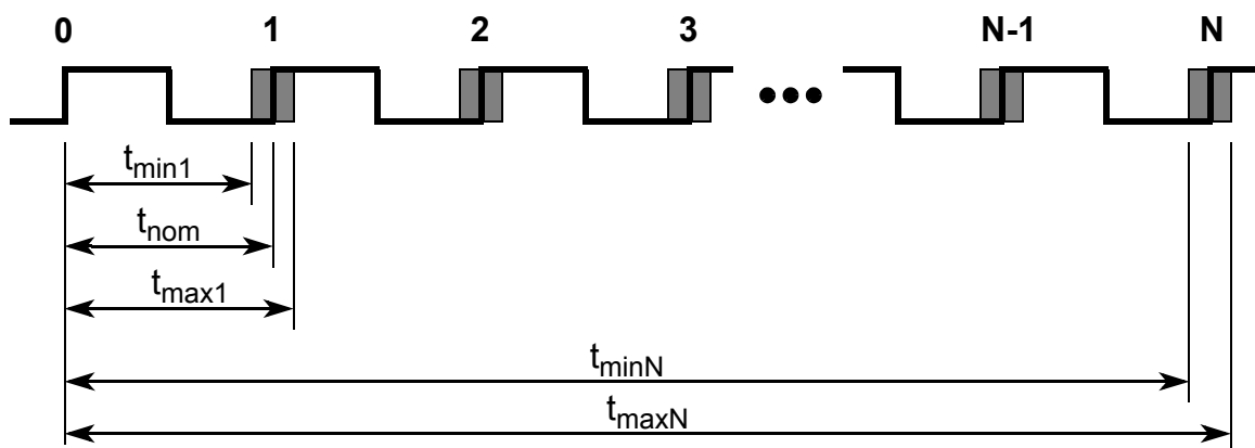
Figure 6. Jitter Definitions
