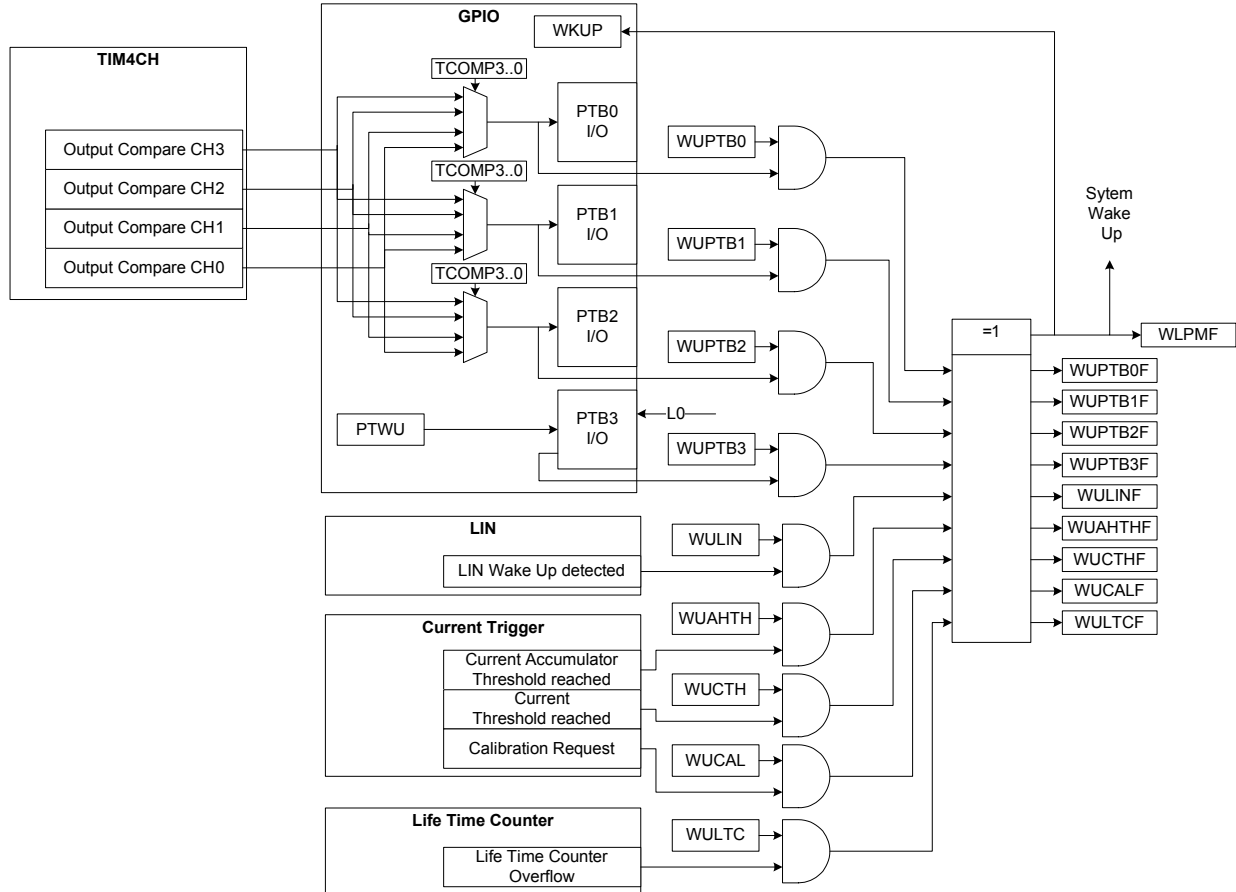
Figure 19. Wake-up Sources
