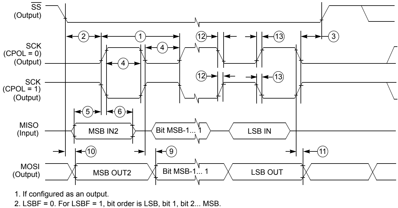
Figure 8. SPI Master Timing (CPHA = 0)
