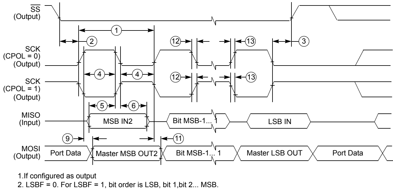
Figure 9. SPI Master Timing (CPHA = 1)
