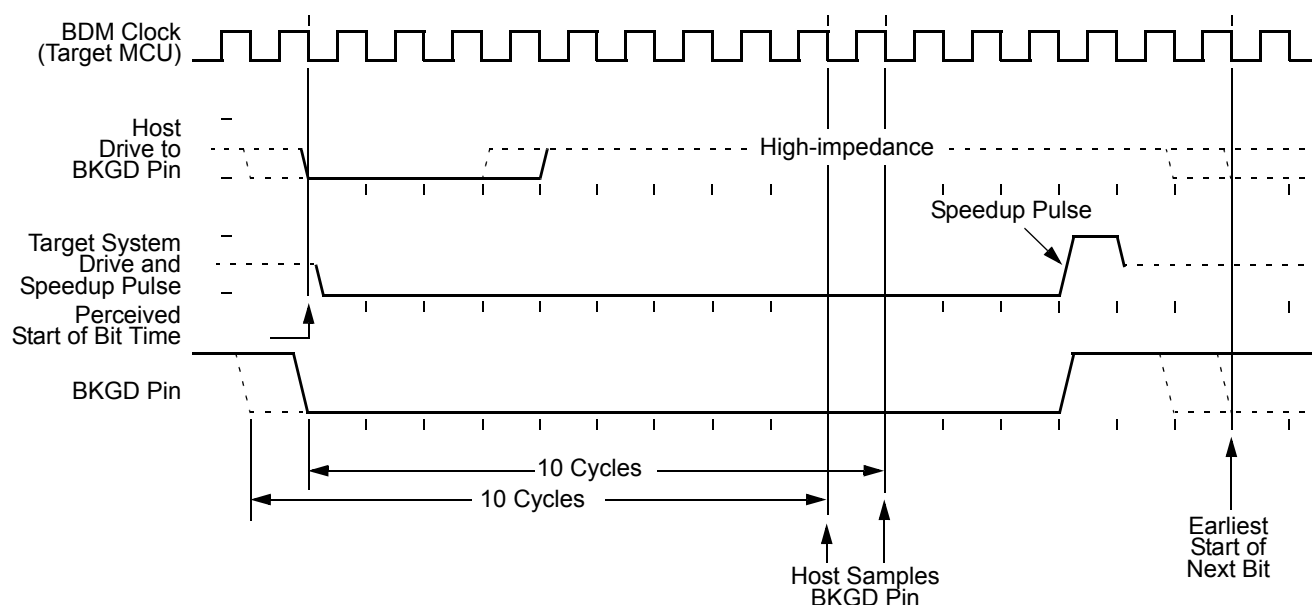
Figure 85. BDM Target-to-Host Serial Bit Timing (Logic 0)
