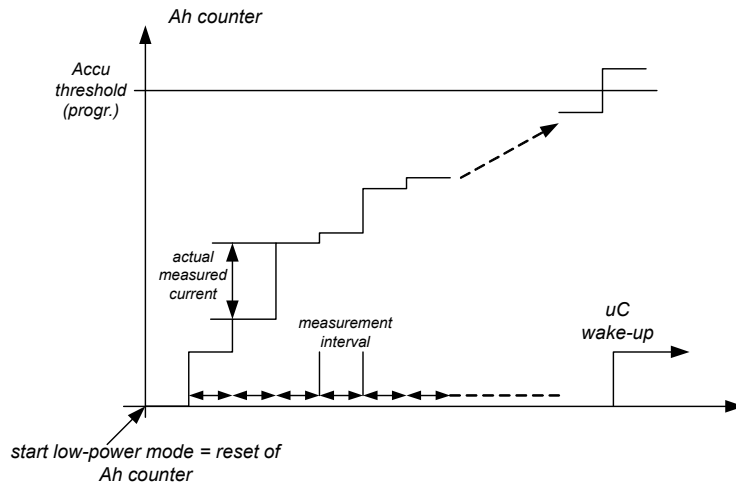
Figure 21. Ah Counter Function
