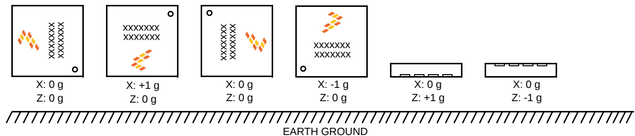
Figure 4. Device orientation diagram
