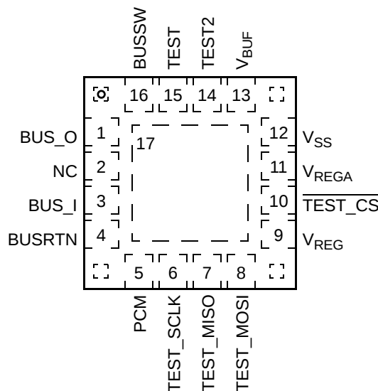
Figure 2. Pin connections
