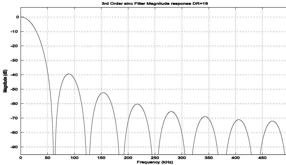
Figure 16. Sinc-filter response
