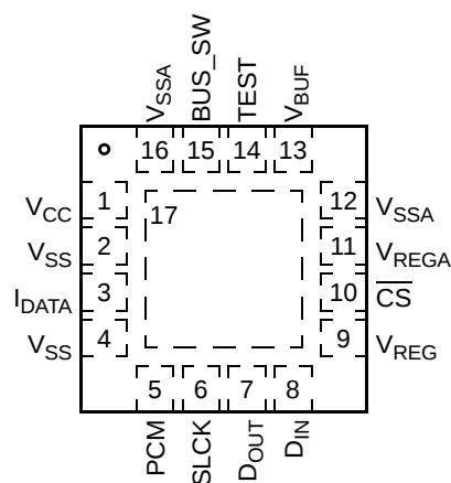
PIN CONNECTIONS
