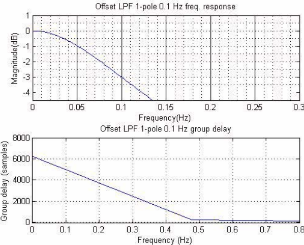
Figure 21. 0.1 Hz Offset Cancellation Low-Pass Filter Characteristics
