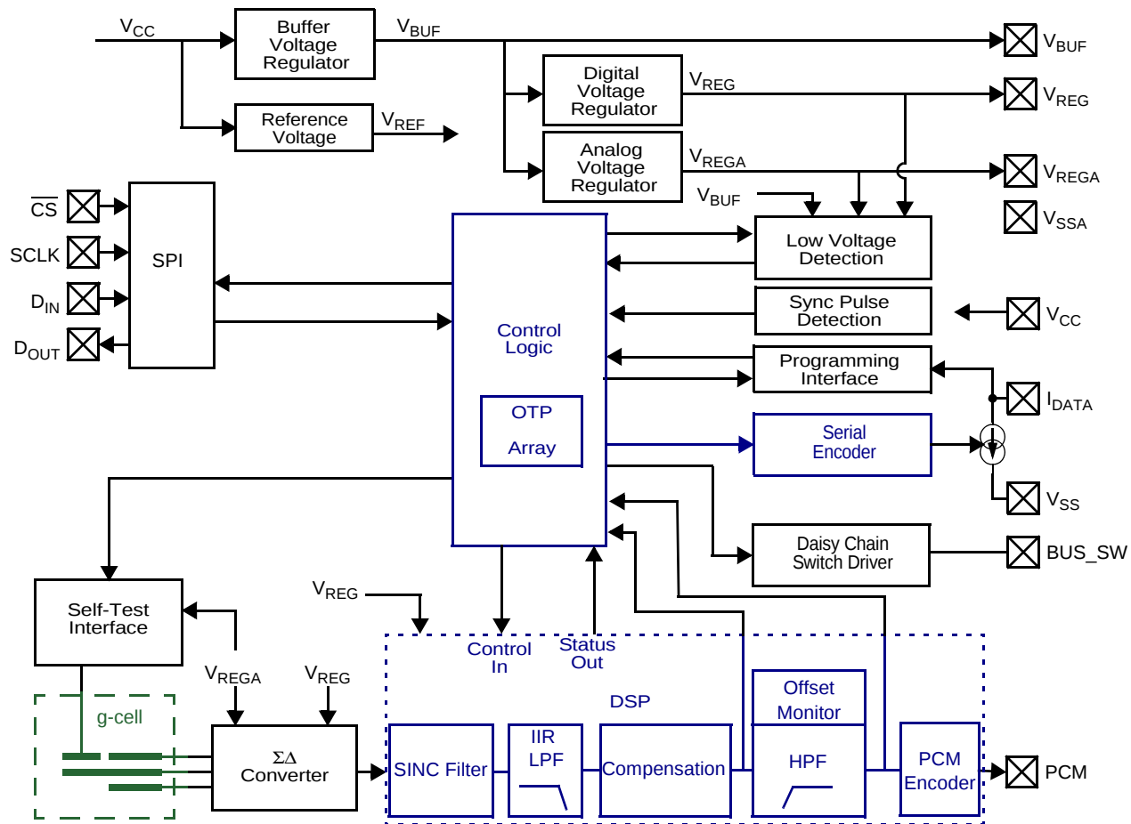
Figure 3. Block Diagram
