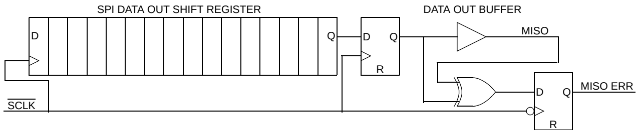
Figure 37. SPI Data Output Verification
