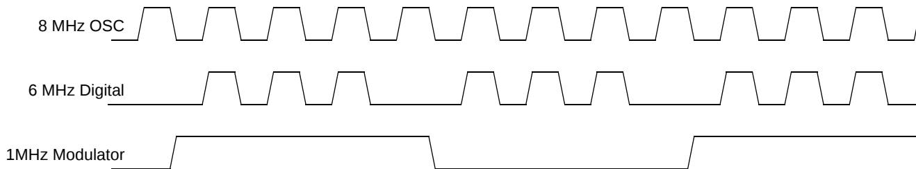
Figure 13. Clock Generation
