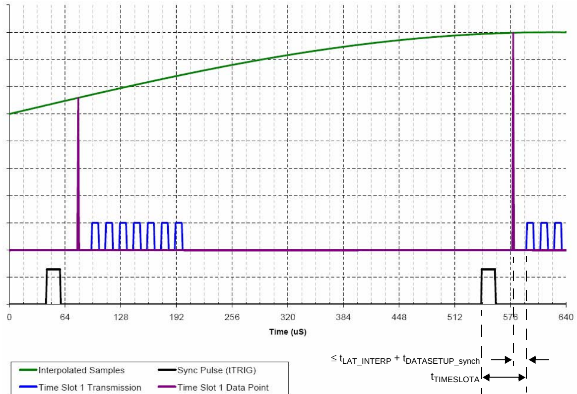
Figure 36. Synchronous Sampling Mode with Minimum Latency
