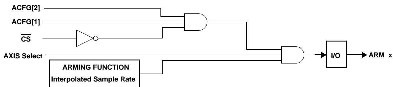
Figure 26. Arming Function Block Diagram - Unfiltered Mode
