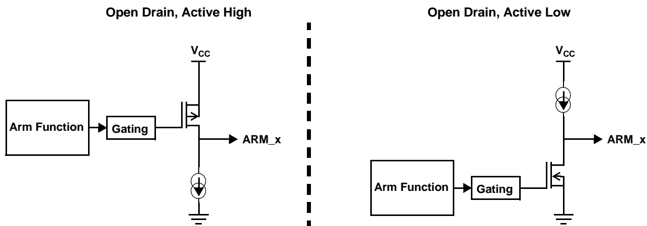
Figure 28. Arming Function - Pin Output Structure
