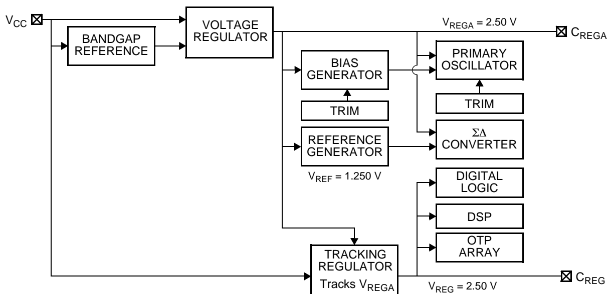
Figure 7. Power Supply
