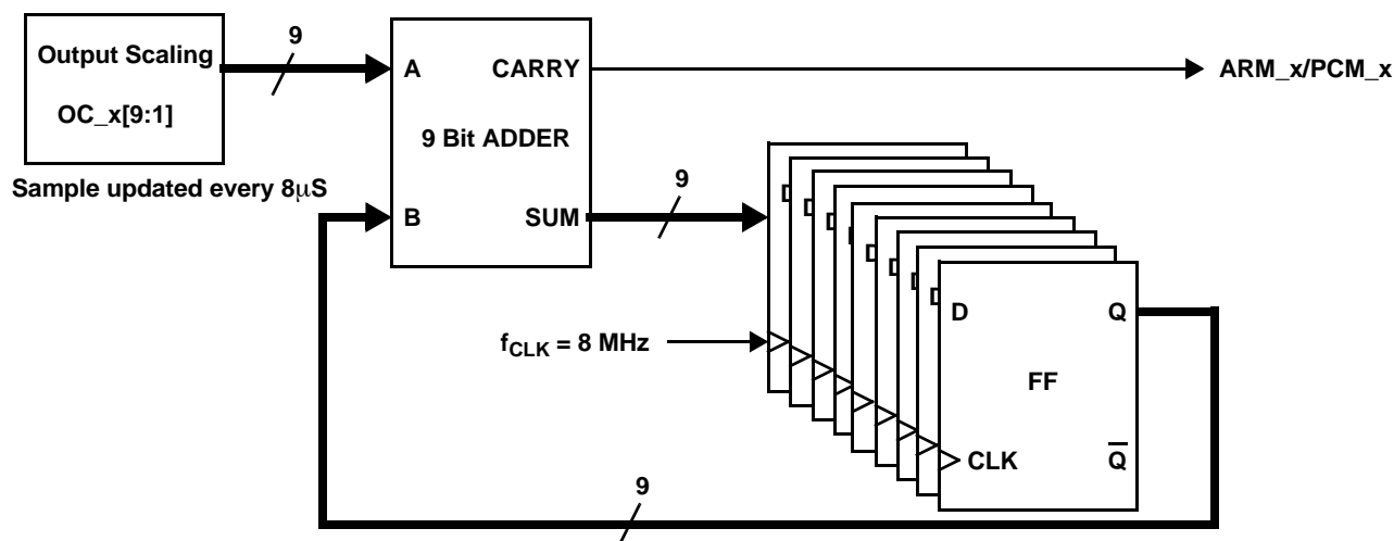
Figure 29. PCM Output Function Block Diagram
