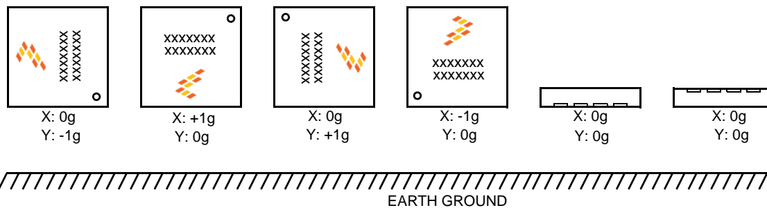
Figure 2. Device Orientation Diagram
