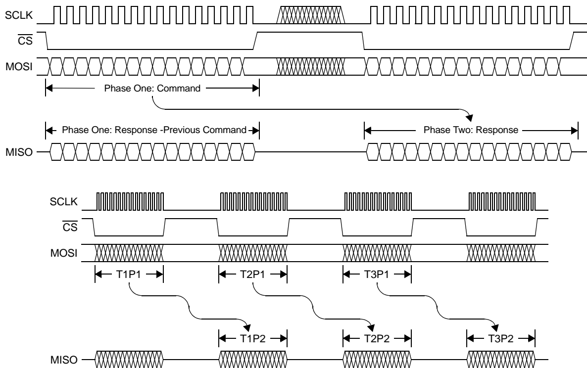
Figure 33. SPI Transfer Detail
