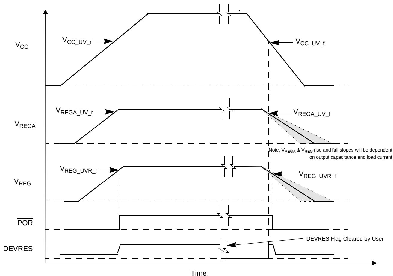
Figure 5. Powerup Timing
