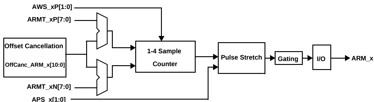
Figure 24. Arming Function Block Diagram - Count Mode
