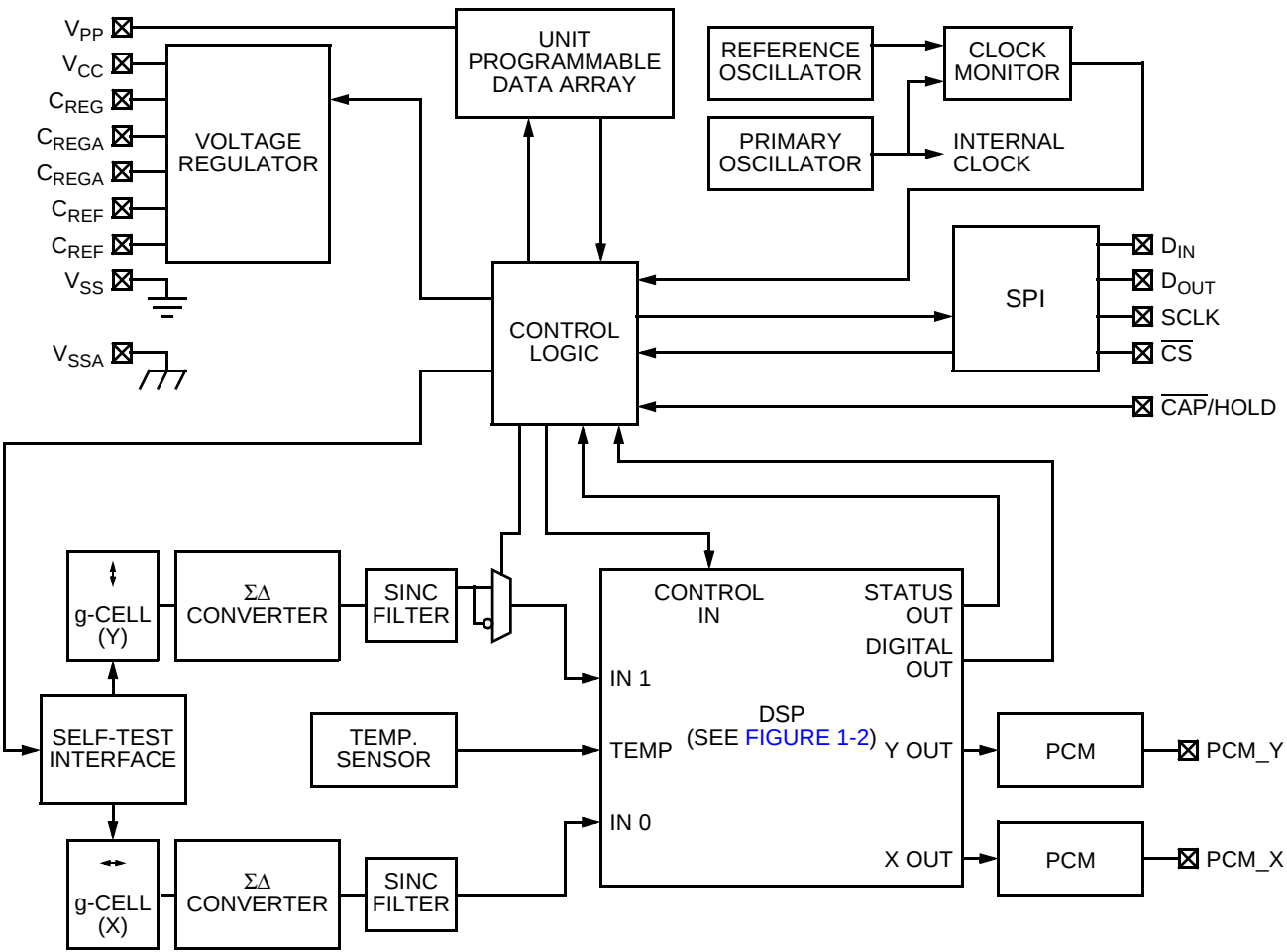
Figure 1-1 Block Diagram
