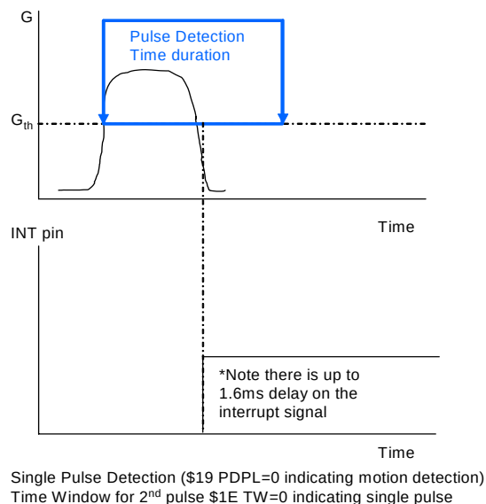
Figure 4. Single Pulse Detection
