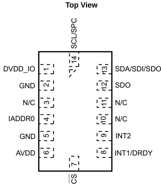
Figure 14. Pinout Description
