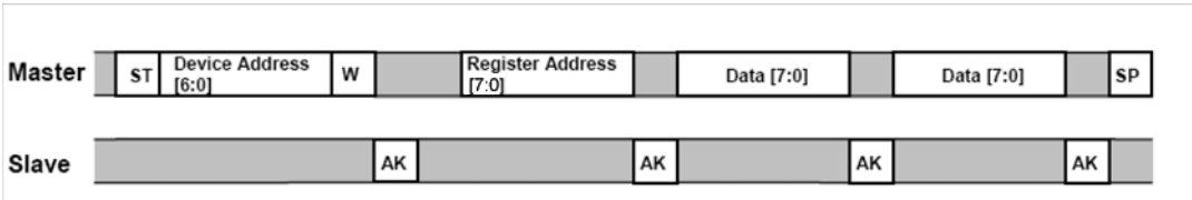
Figure 10. Multiple Byte Writes - The Master (MCU) is writing to multiple sequential registers of the MMA7455L
