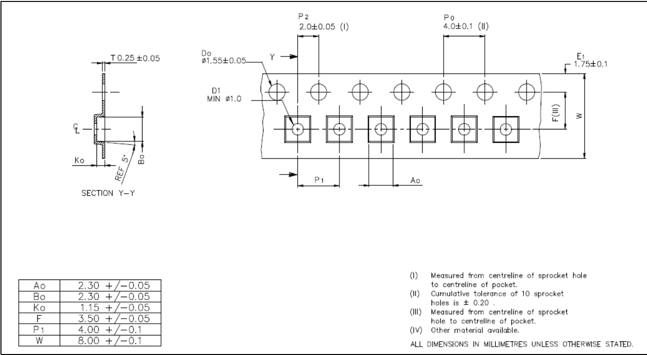
Figure 47. Carrier tape
