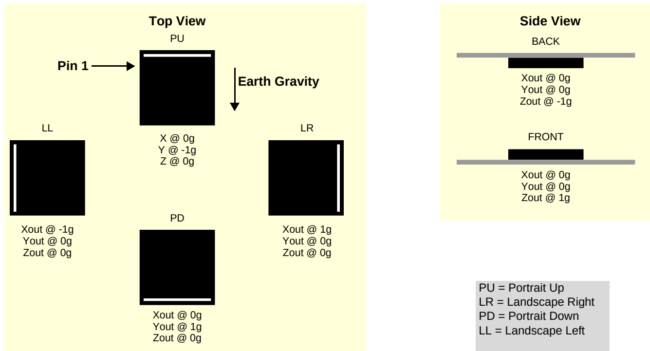
Figure 3. Landscape/Portrait orientation
