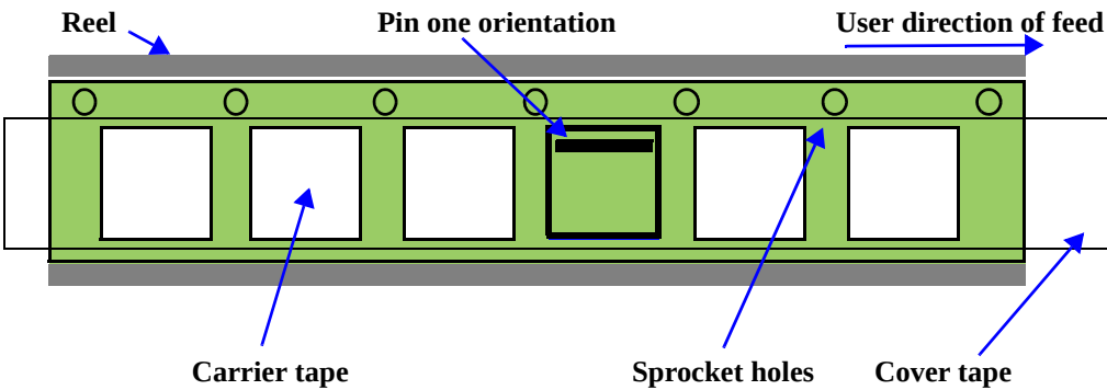
Figure 48. Device orientation on carrier tape
