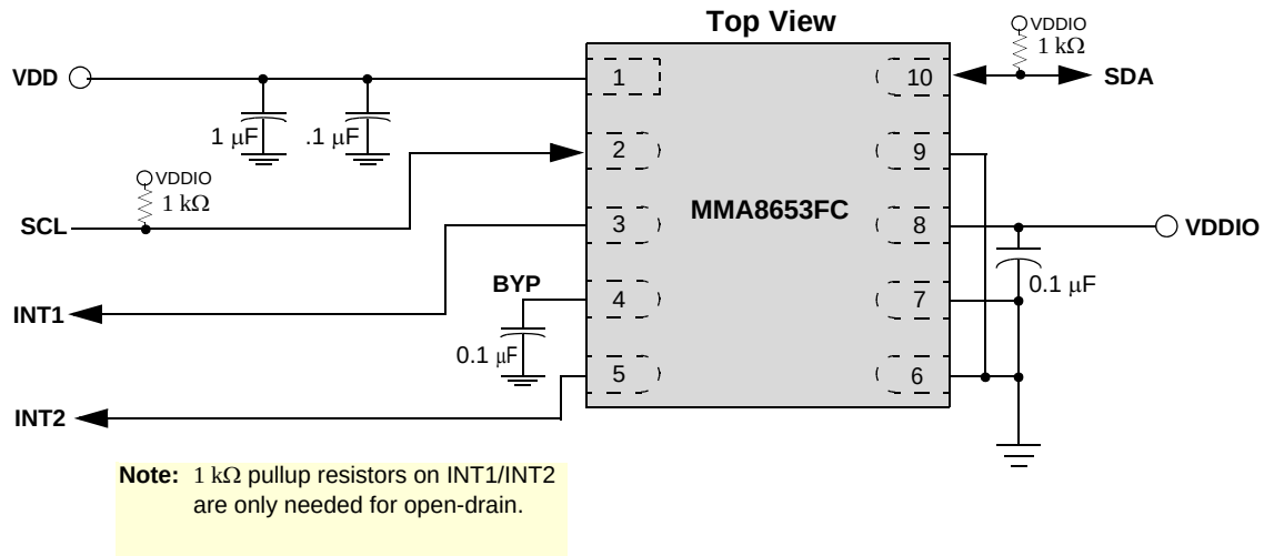
Figure 4. Application diagram
