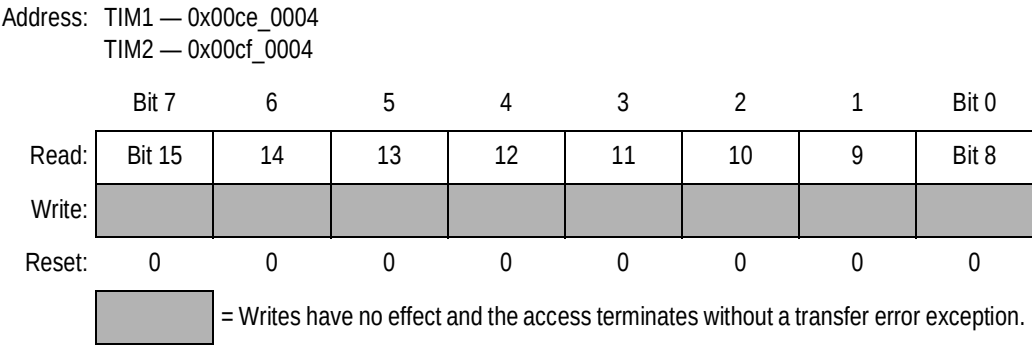
Figure 16-6. Timer Counter Register High (TIMCNTH)
