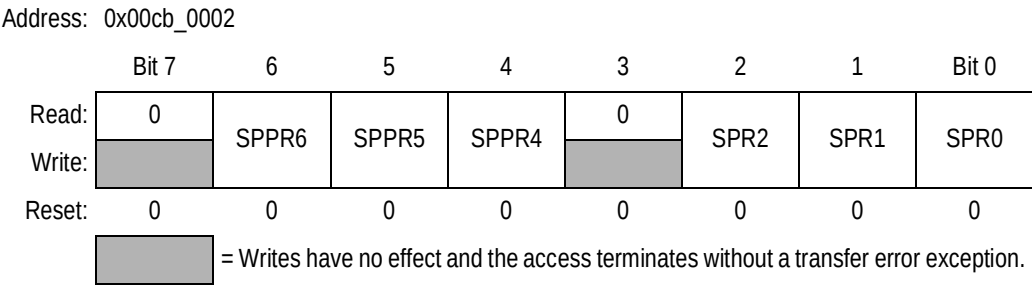
Figure 18-4. SPI Baud Rate Register (SPIBR)
