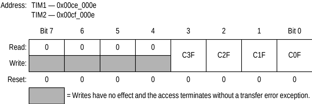
Figure 16-15. Timer Flag Register 1 (TIMFLG1)
