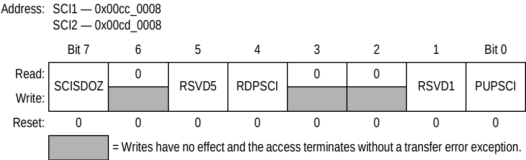
Figure 17-10. SCI Pullup and Reduced Drive Register (SCIPURD)
