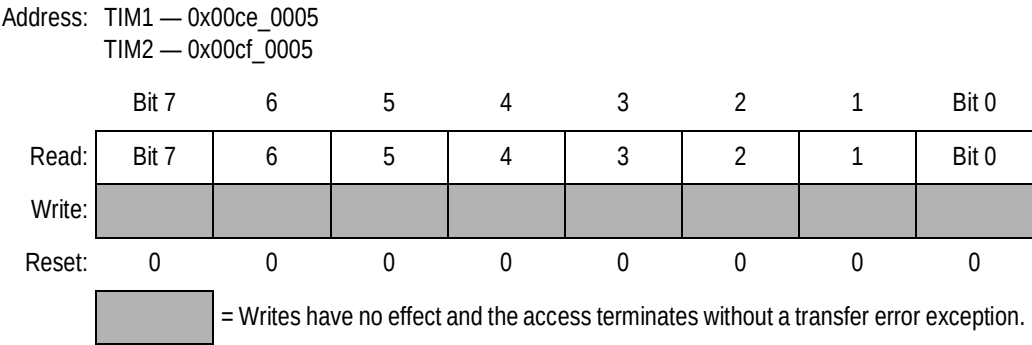
Figure 16-7. Timer Counter Register Low (TIMCNTL)
