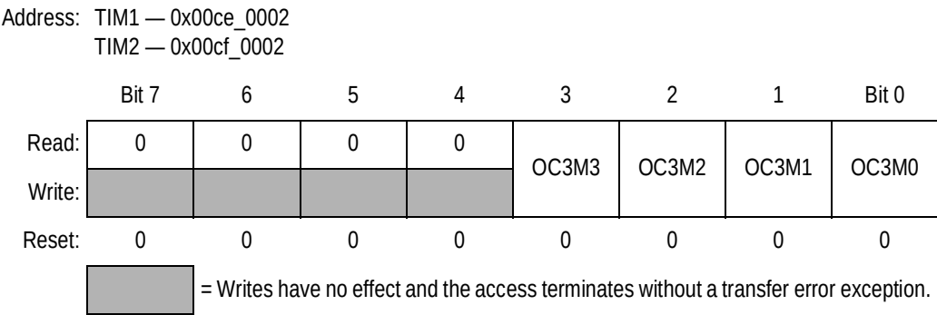
Figure 16-4. Timer Output Compare 3 Mask Register (TIMOC3M)
