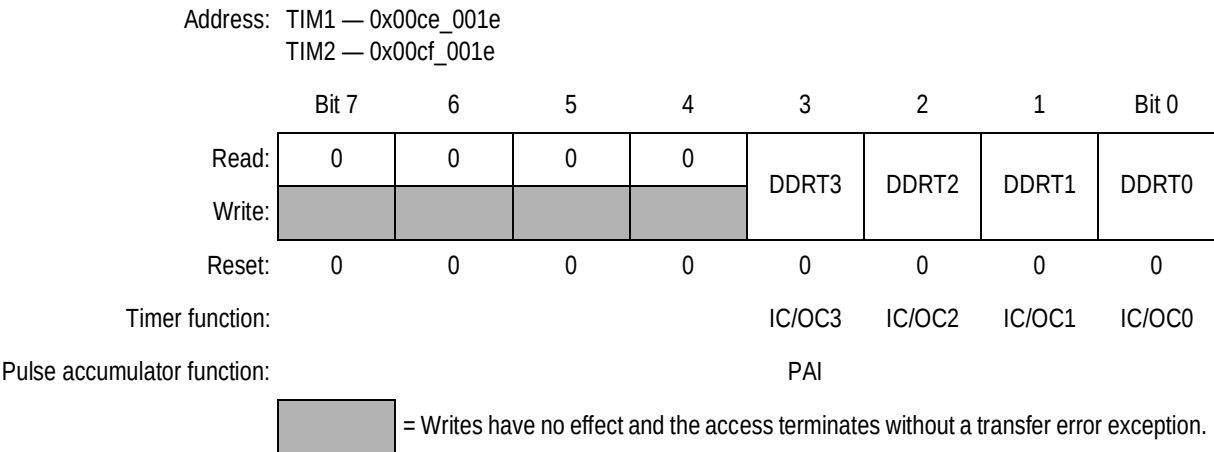
Figure 16-24. Timer Port Data Direction Register (TIMDDR)
