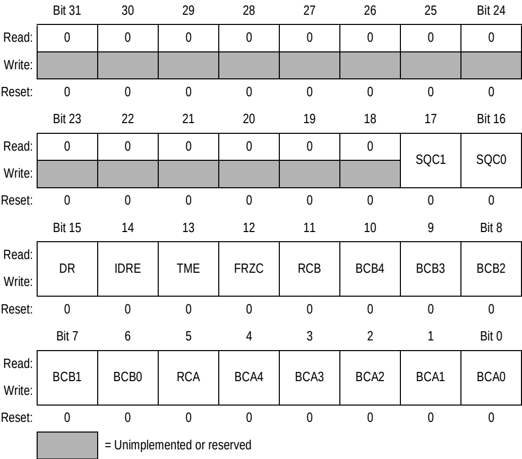
Figure 22-10. OnCE Control Register (OCR)
