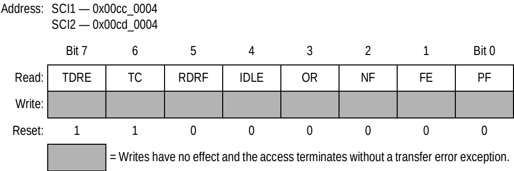
Figure 17-6. SCI Status Register 1 (SCISR1)
