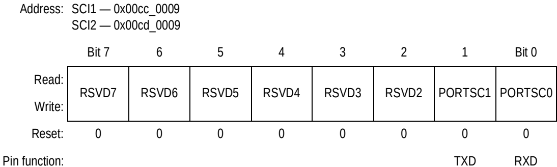
Figure 17-11. SCI Port Data Register (SCIPORT)
