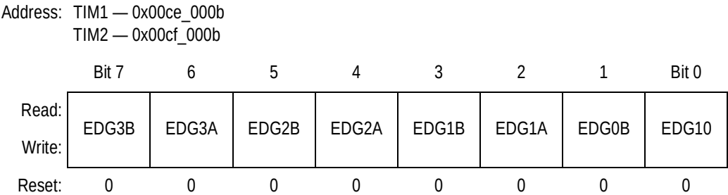
Figure 16-12. Timer Control Register 2 (TIMCTL2)
