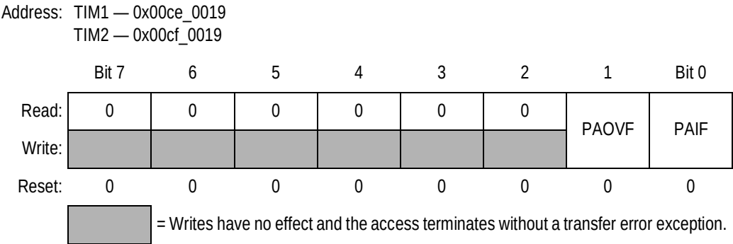
Figure 16-20. Pulse Accumulator Flag Register (TIMPAFLG)
