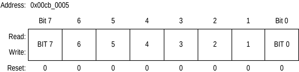
Figure 18-6. SPI Data Register (SPIDR)
