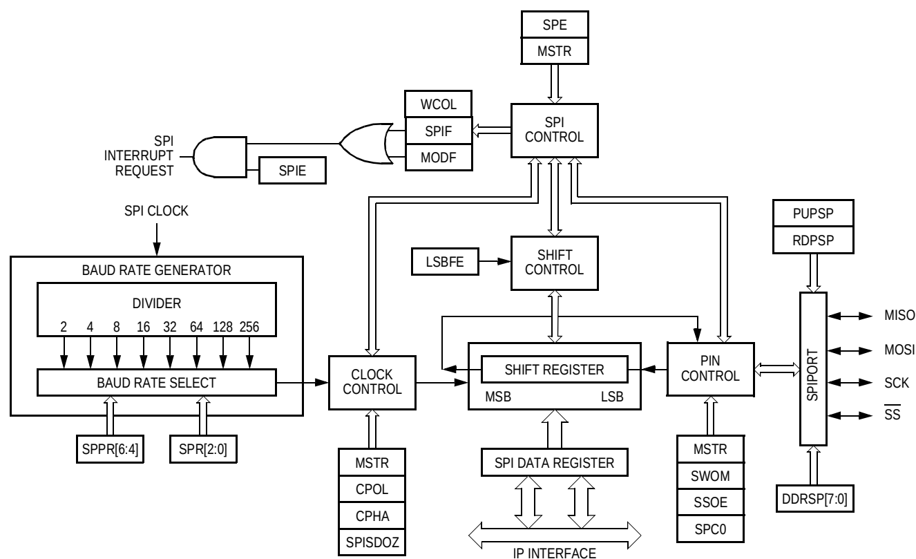
Figure 18-1. SPI Block Diagram
