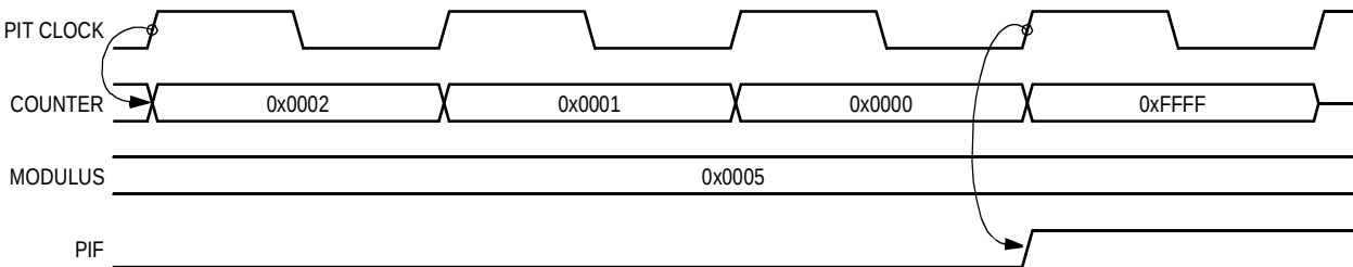
Figure 15-6. Counter in Free-Running Mode
