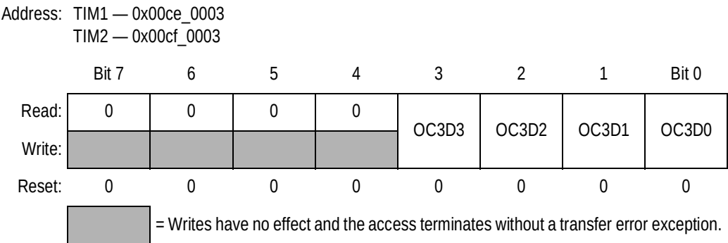
Figure 16-5. Timer Output Compare 3 Data Register (TIMOC3D)
