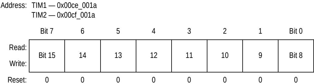
Figure 16-21. Pulse Accumulator Counter Register High (TIMPACNTH)
