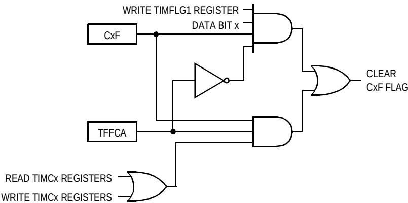
Figure 16-9. Fast Clear Flag Logic
