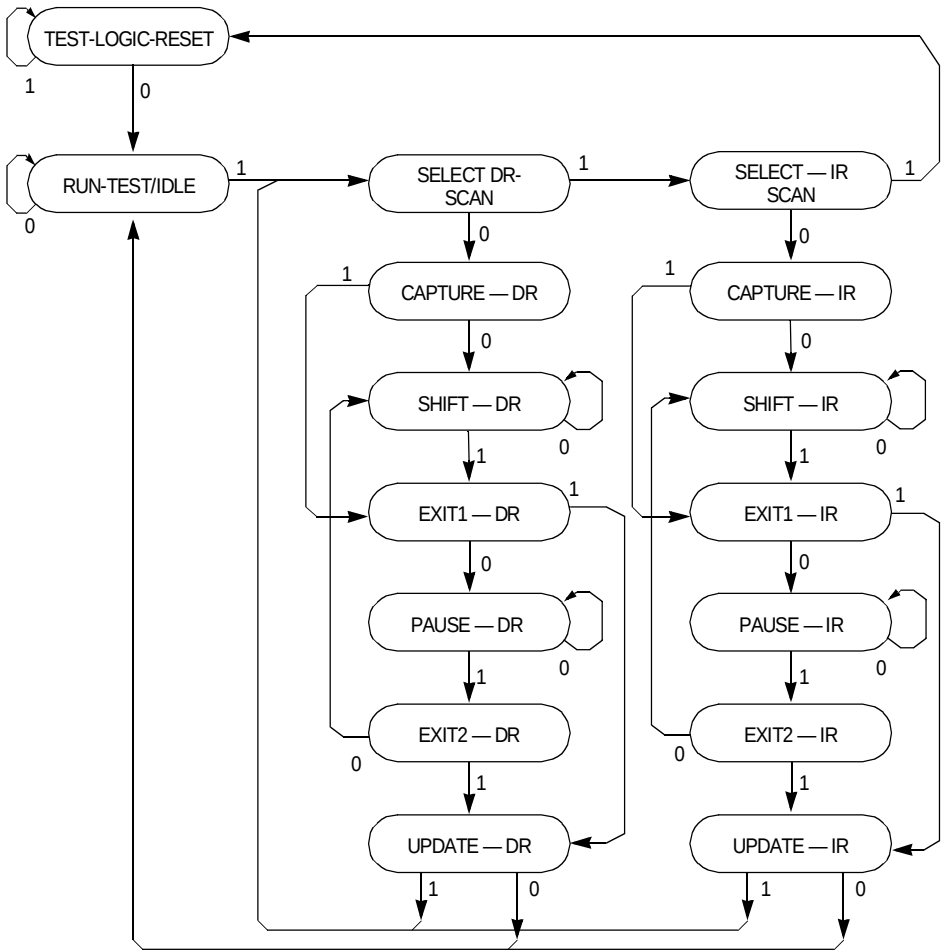
Figure 22-6. OnCE Controller
