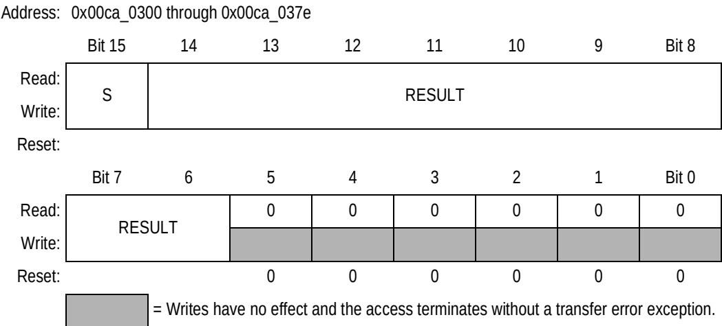
Figure 19-16. Left-Justified Signed Result Register (LJSRR)
