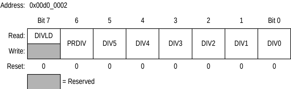
Figure 10-4. SGFM Clock Divider Register (SGFMCLKD)
