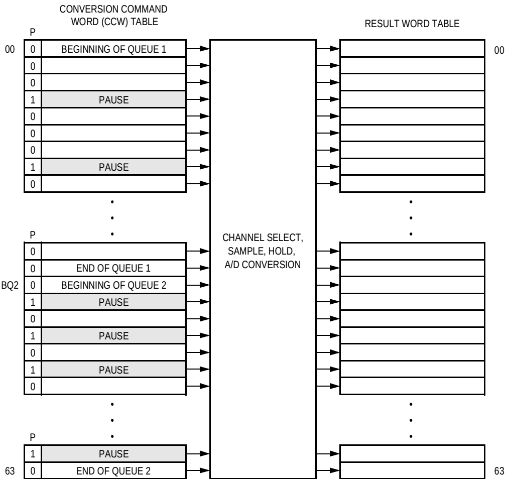
Figure 19-22. QADC Queue Operation with Pause
