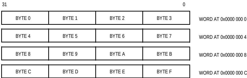
Figure 7-3. Data Organization in Memory
