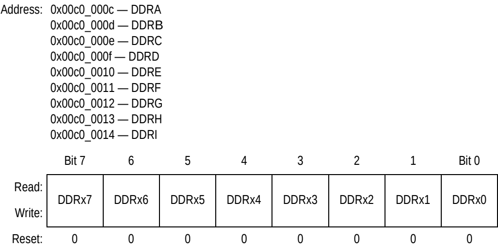
Figure 12-3. Port Data Direction Registers (DDRx)
