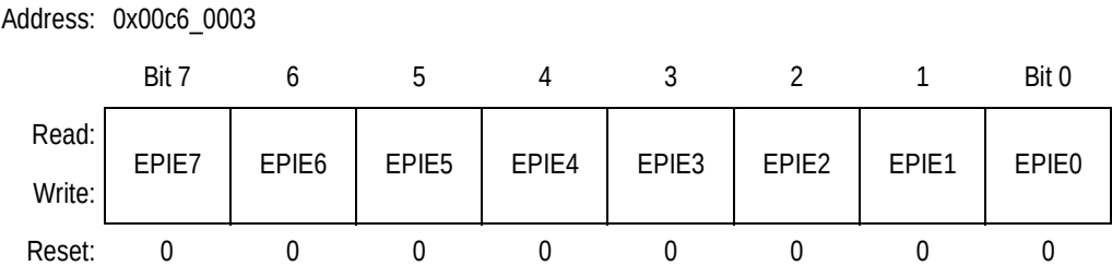
Figure 13-4. EPORT Port Interrupt Enable Register (EPIER)
