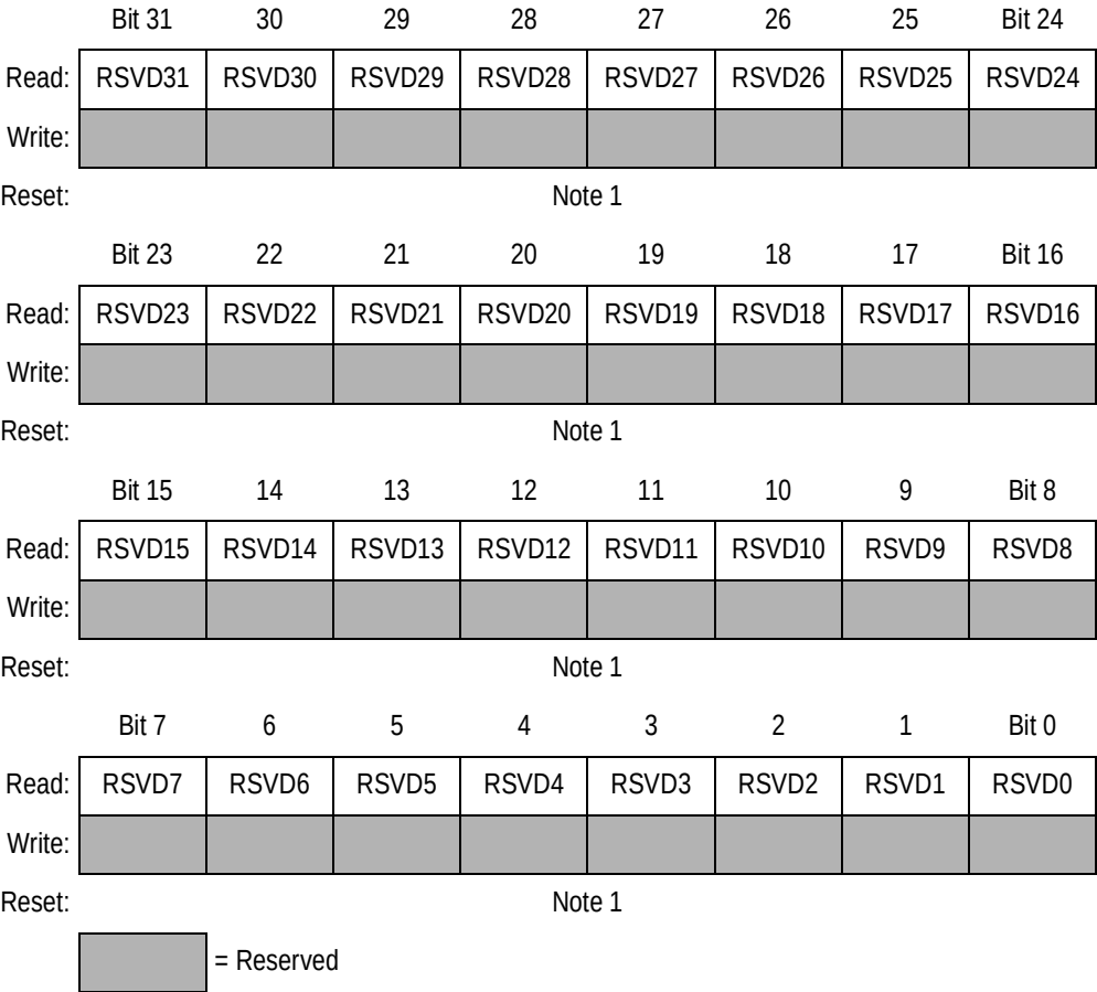
Figure 10-7. SGFM Monitor Data Register (SGFMMNTR)
