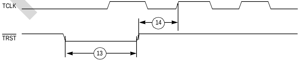
Figure 23-11. \overline{\text{TRST}} Timing
