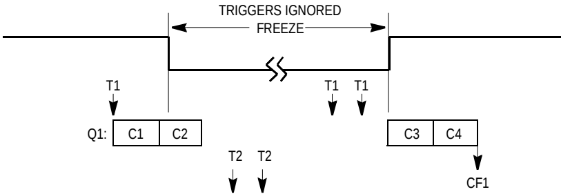
Figure 19-36. CCW Freeze Situation 14
