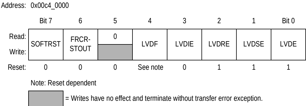
Figure 5-2. Reset Control Register (RCR)
