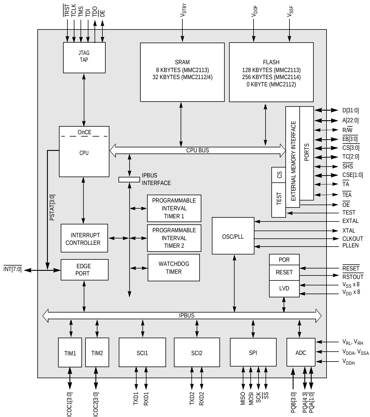
Figure 1-1. Block Diagram
