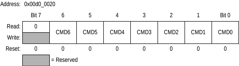
Figure 10-14. SGFM Command Register (SGFMCMD)
