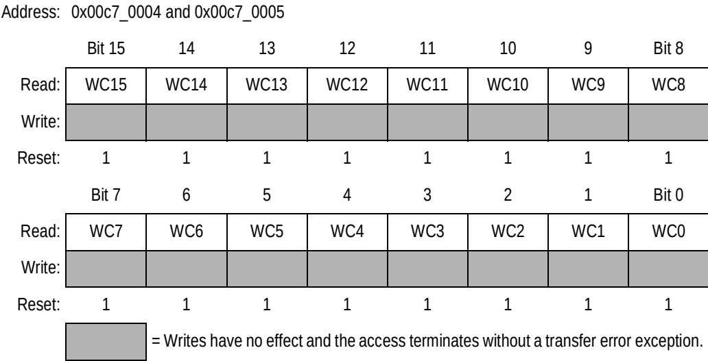
Figure 14-4. Watchdog Count Register (WCNTR)
