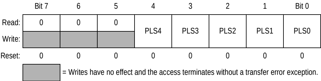
Figure 8-11. Priority Level Select Registers (PLSR0–PLSR39)
