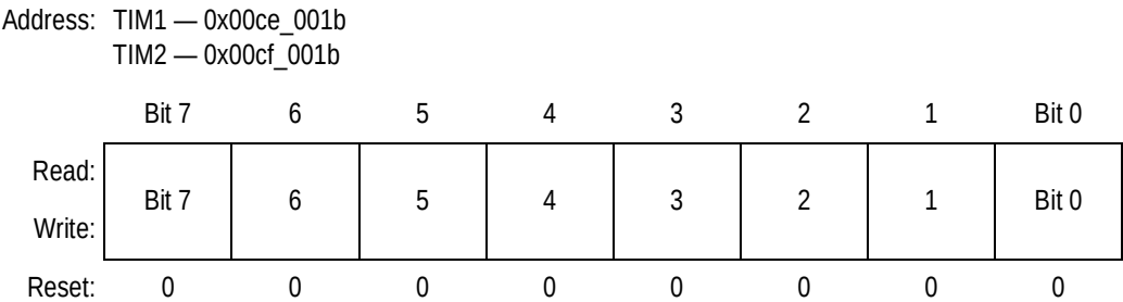
Figure 16-22. Pulse Accumulator Counter Register Low (TIMPACNTL)
