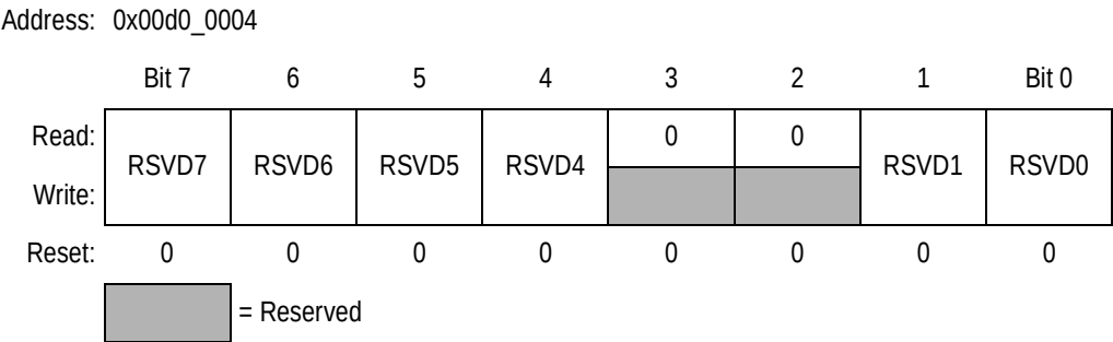
Figure 10-5. SGFM Test Register (SGFMTST)
