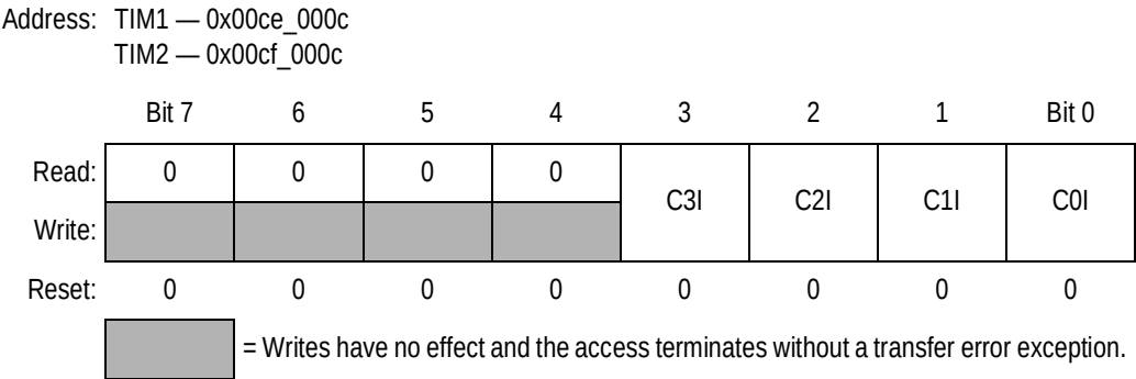
Figure 16-13. Timer Interrupt Enable Register (TIMIE)
