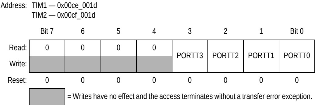
Figure 16-23. Timer Port Data Register (TIMPORT)
