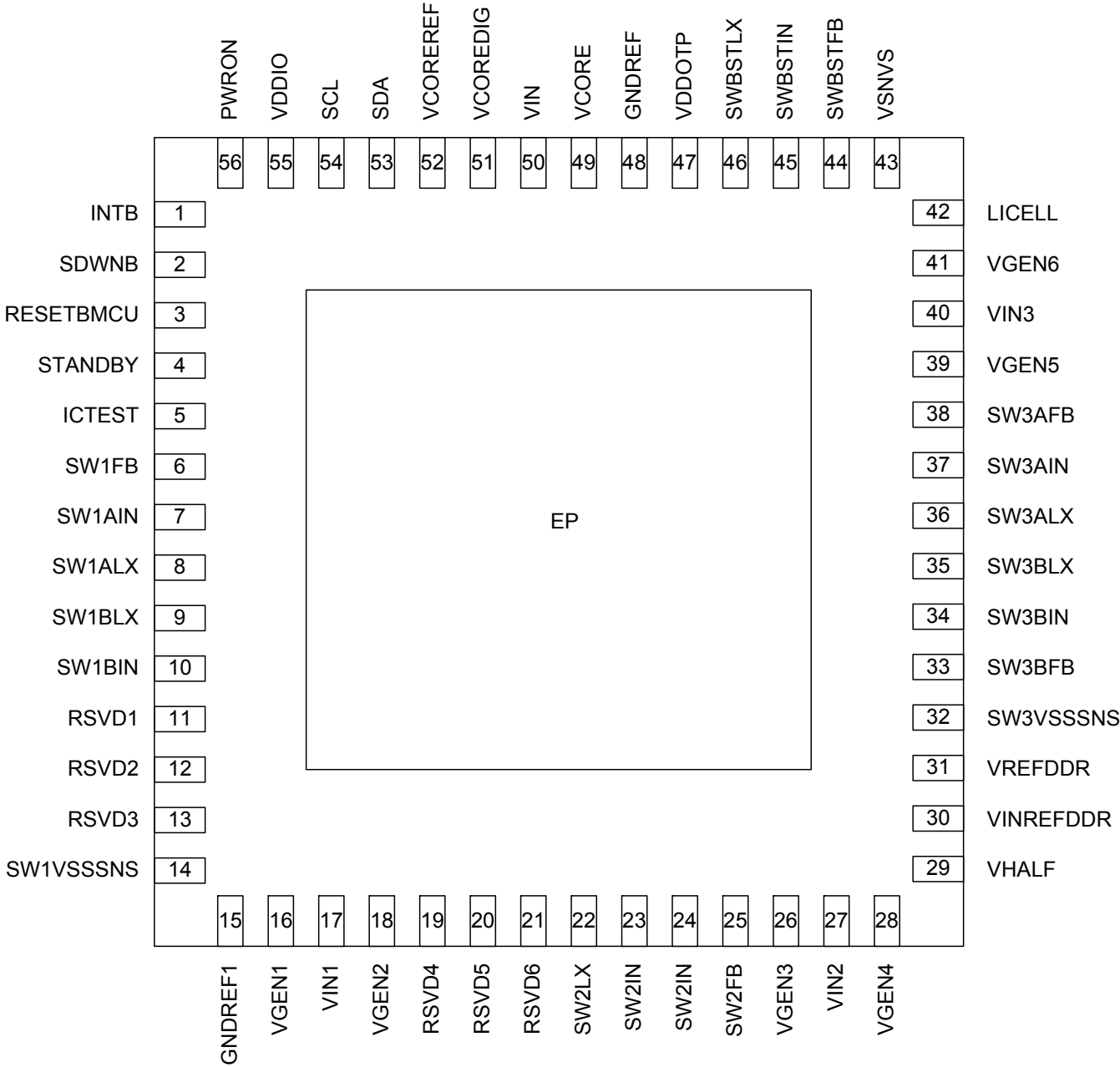
Figure 3. Pinout Diagram
