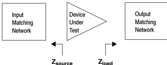
Figure 12. Series Equivalent Source and Load Impedance
