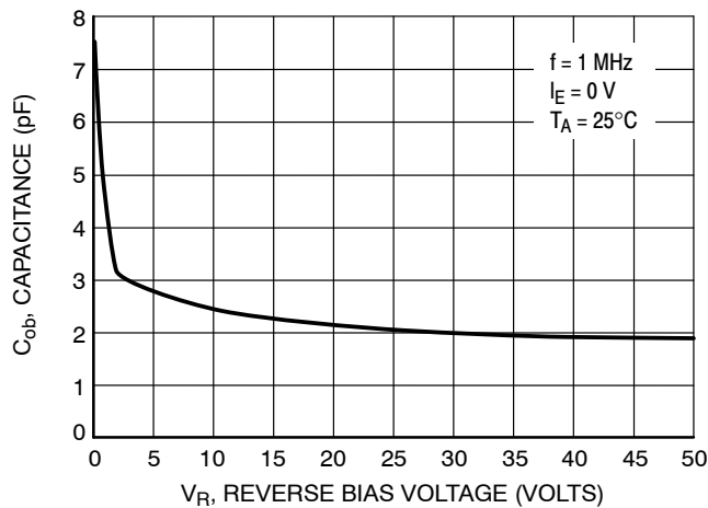
Figure 39. Output Capacitance
