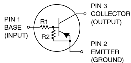
SOT-23 CASE 318 STYLE 6
