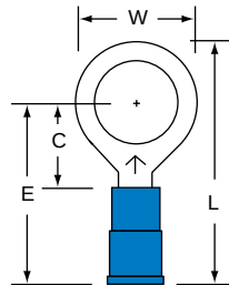
MNG14-38R Stud Size 3/8 Wire Range 16-14
