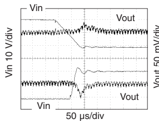
MOR2815S Step Line Response FIGURE 39
