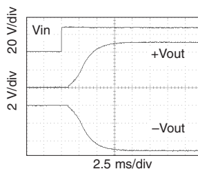
MOR2805D Turn On Response
