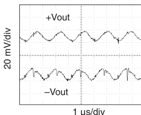
MOR2812D Output Ripple ( \pm Vout)
