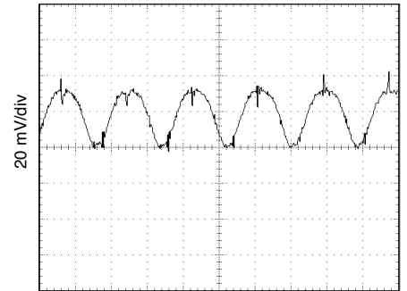
1 μs/div MOR2815S Output Ripple (Vout) FIGURE 37
