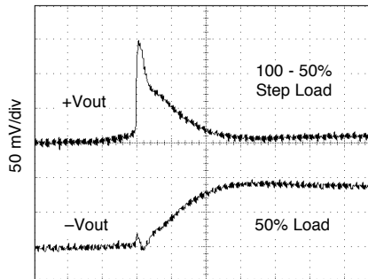
50 μs/div MOR2805D Step Load Response
