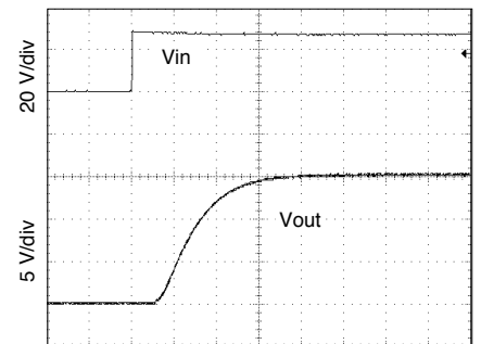
2.5 ms/div All combinations of line and load MOR2815S Turn On Response FIGURE 40
