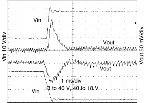
MOR2805S Step Line Response FIGURE 32
