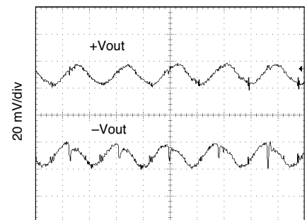
MOR2812D Output Ripple (±Vout)
