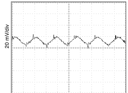
80% Load MOR2805S Output Ripple (Vout)
