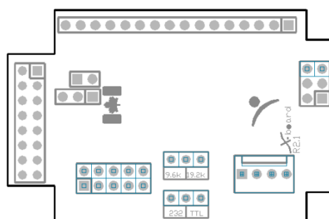
Figure 2: MOS X-Board
