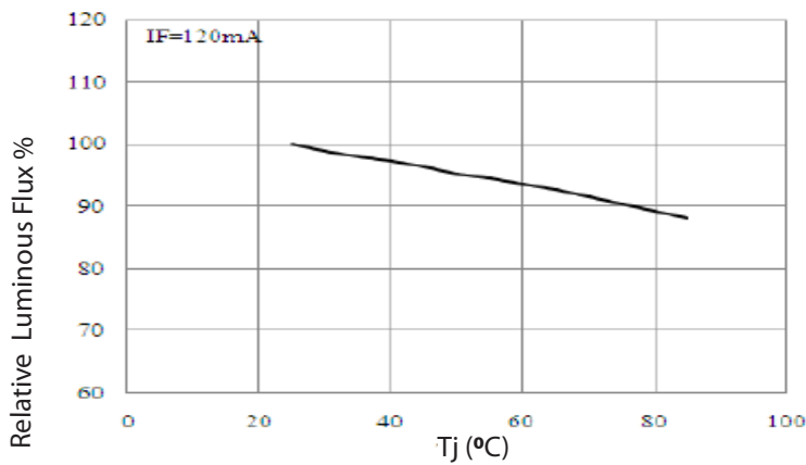
Tj-----Relative Luminous Flux
