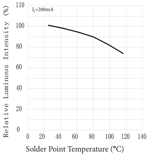
T_s --Relative Luminous flux
