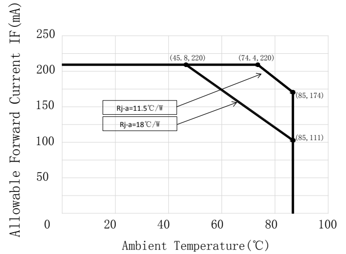
Ambient Temperature- Allowable Forward Current
