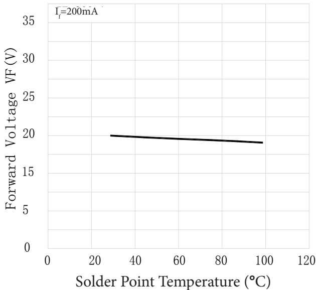
T_s ----Forward Voltage
