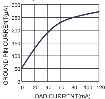
Ground Pin Current vs. Output Current
