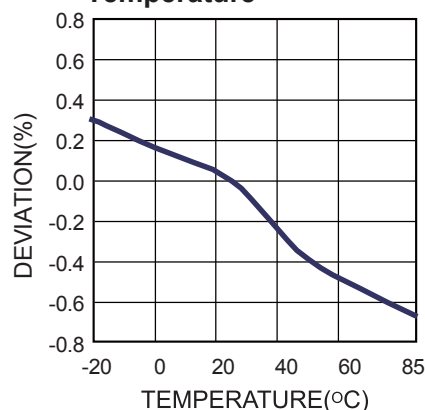
Voltage Accuracy vs. Temperature
