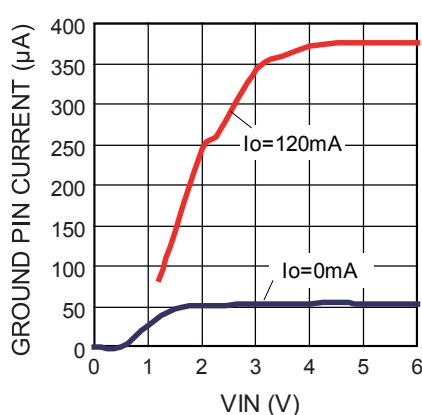
Ground Pin Current vs. V_{IN}
