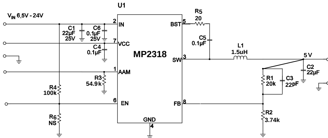
Figure 10: V_{in}=19V , V_o=5V , I_o=2A
