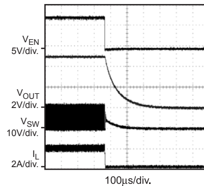
Shutdown I_{OUT} = 2A
