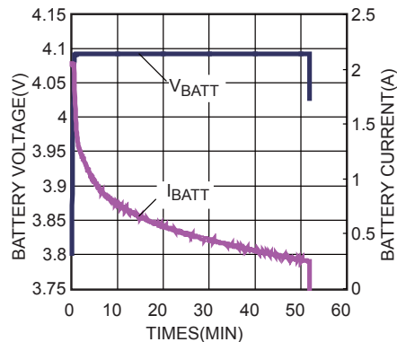
1-Cell Battery Charge Curve
