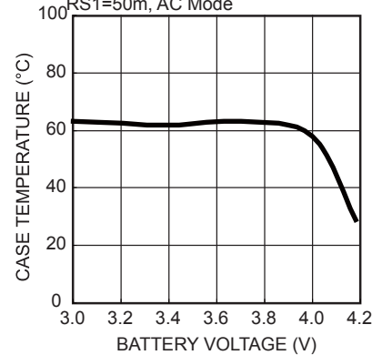
Case Temperature vs. Battery Voltage
