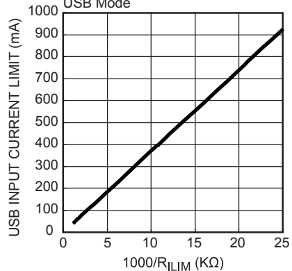
USB Input Current Limit vs. 1000/R_{ILIM}
