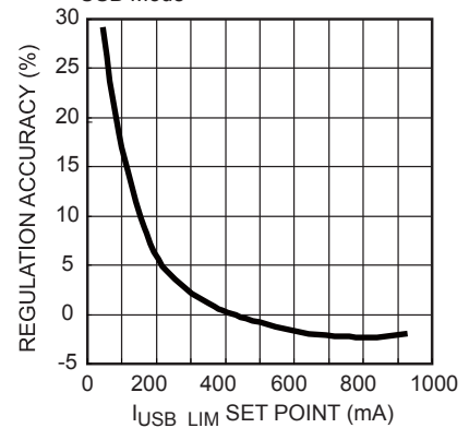
USB Input Current Limit Accuracy
