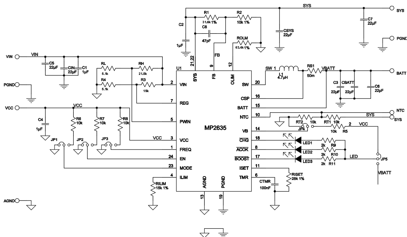
Figure 14: The detailed application circuit of MP2635
