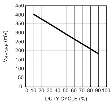
Figure 2— V_{SENSE} vs Duty Cycle
