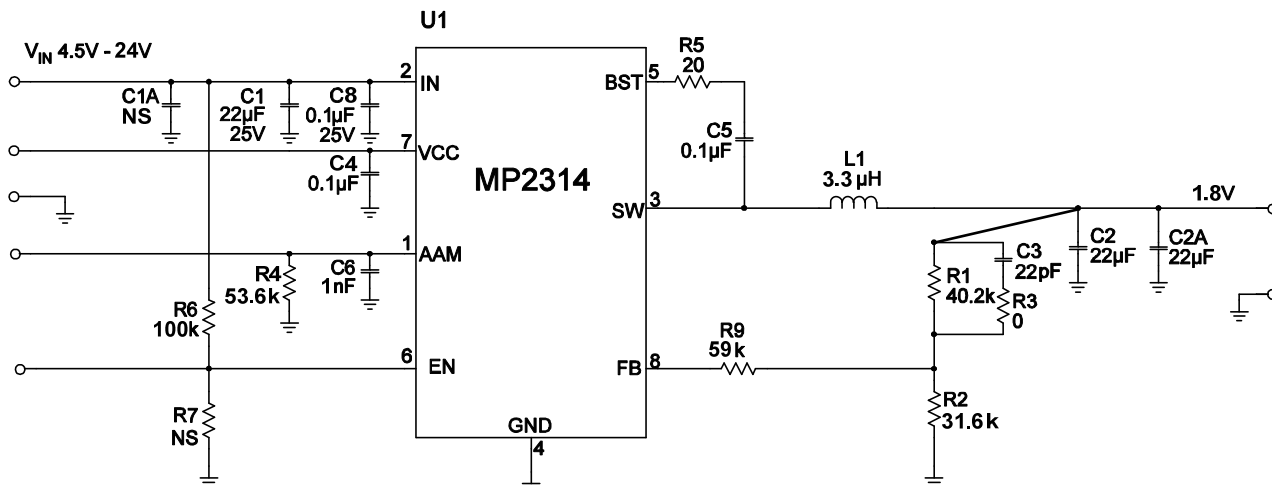
Figure 12: Vo=1.8V, Io=2A
