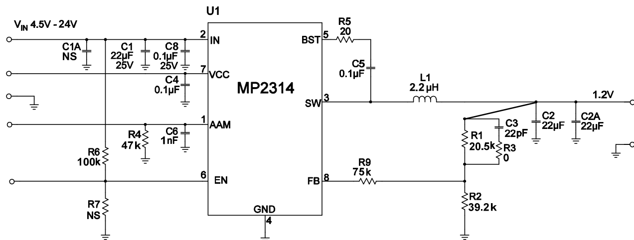
Figure 13: Vo=1.2V, Io=2A
