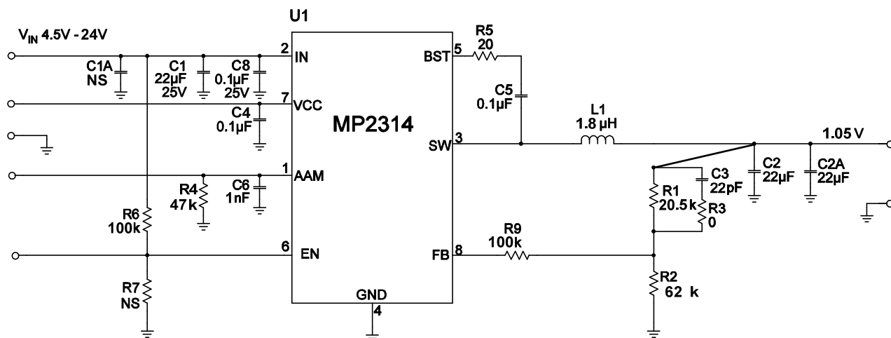
Figure 14: Vo=1.05V, Io=2A
