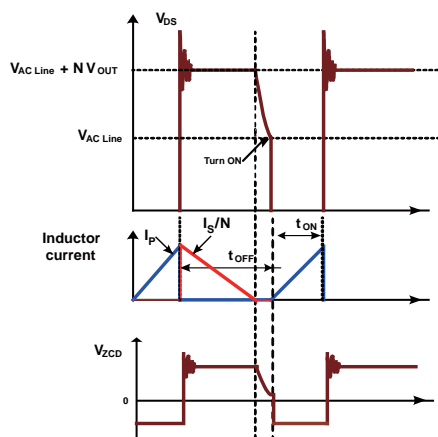
Figure 2: Boundary-Conduction Mode
