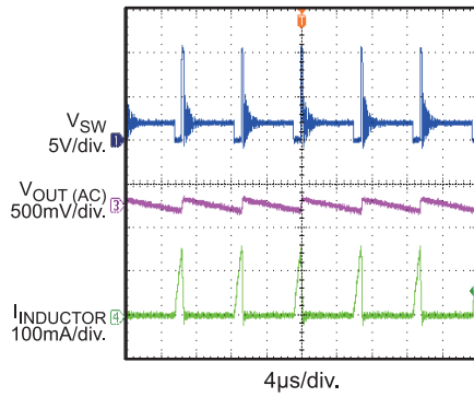
Steady State Waveforms V_{IN}=2V
