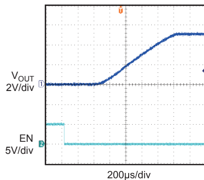
Turn On Delay and Rise Time with 0.22 \mu F Load
