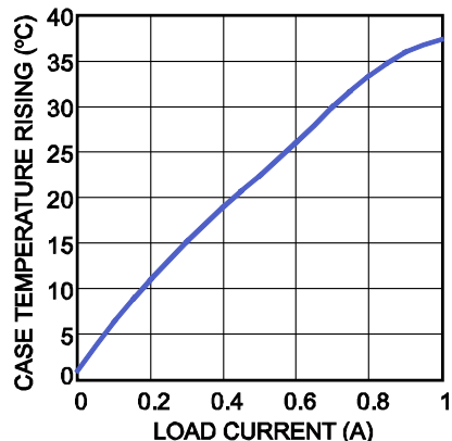
Case Temperature Rising vs. Load Current
