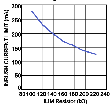
PD Inrush Current Limit vs. Setting Resistor
