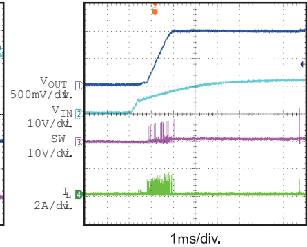
Start Up Through I_{IN} I_{OUT}=0
