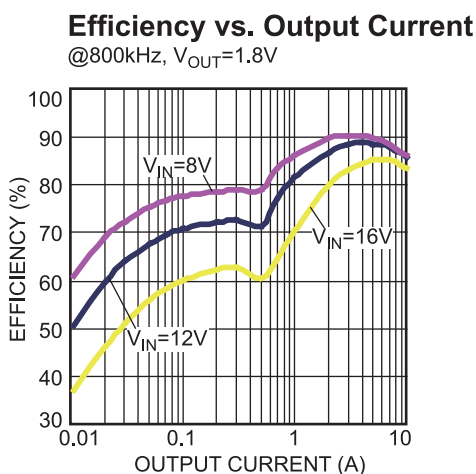
Figure 42 — Efficiency Curve
