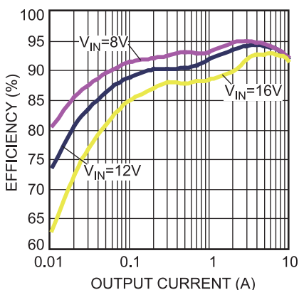
Figure 46 — Efficiency Curve
