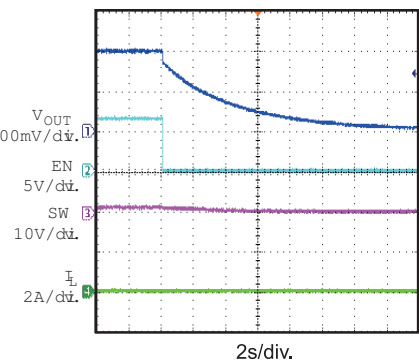
Shutdown Through EN I_{OUT}=0
