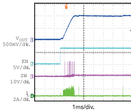
Start up through EN I_{OUT}=0
