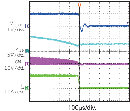
Shutdown Through I_{IN} I_{OUT}=10A
