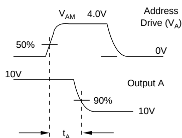
ACCESS TIME WAVEFORM
