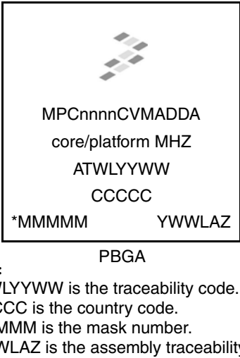
Figure 56. Freescale Part Marking for PBGA Devices
