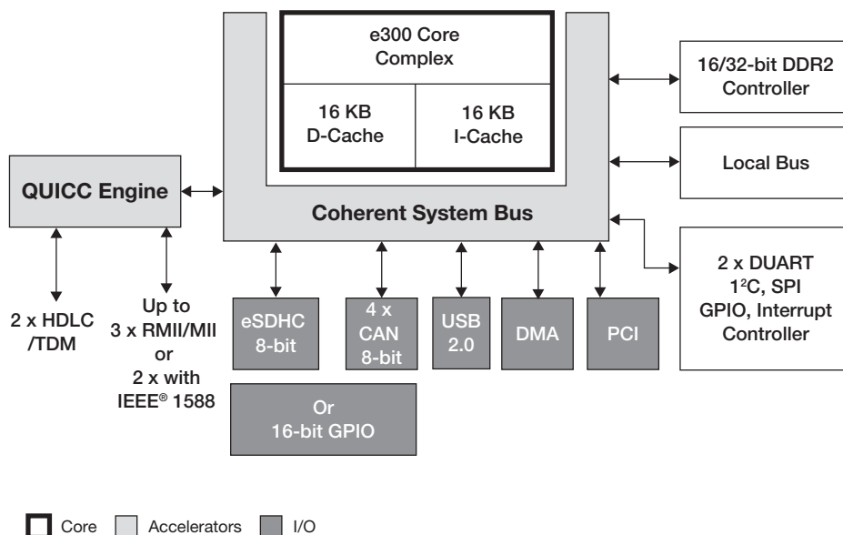
MPC8309 Block Diagram
