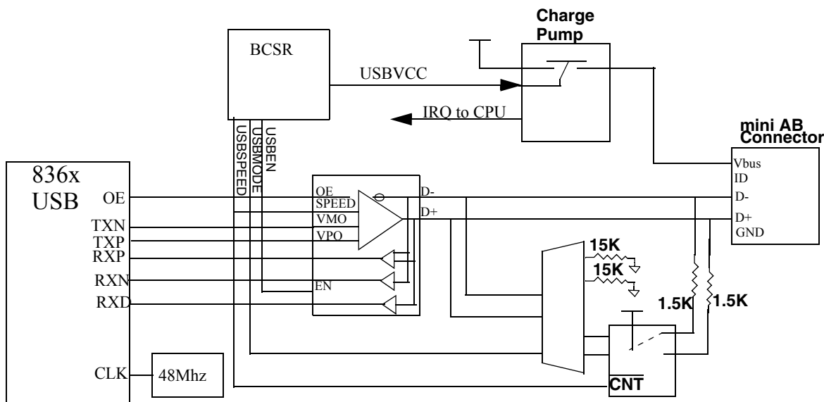
Figure 5-15. USB 1.1 Block
