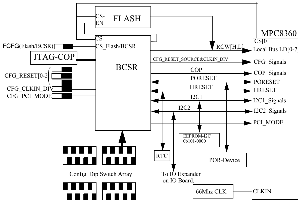
Figure 5-1. Reset Circuit Block Diagram
