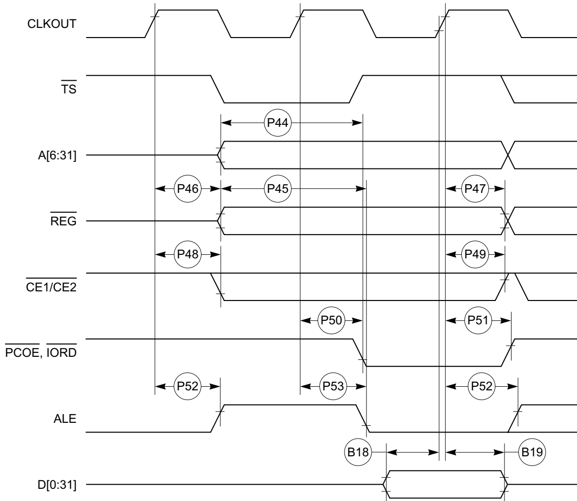
Figure 6-24. PCMCIA Access Cycles Timing External Bus Read
