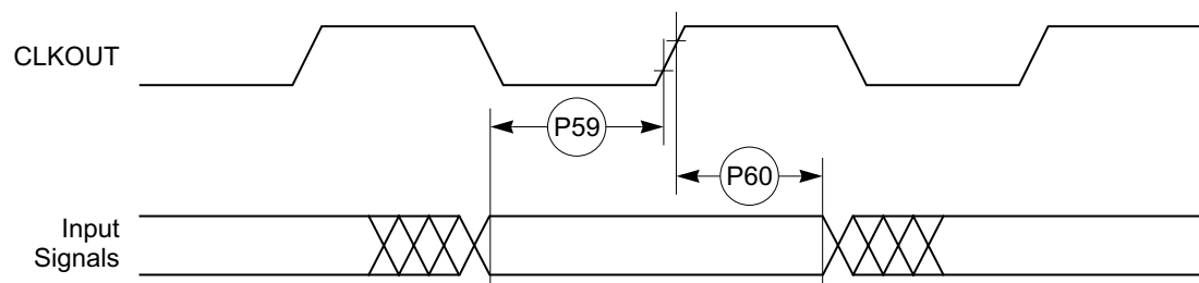
Figure 6-28. PCMCIA Input Port Timing
